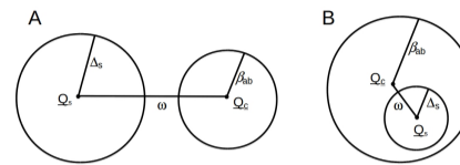
Fig. 5. Schematic illustration of two important angular relationships in the branch-and-bound search. (A) The case of \omega > \beta_{ab} + \Delta_s in sub-cube s of the \pi -ball. In this case, the clash rotation, \underline{R}_c^{ab} , cannot fall within the rotation volume of sub-cube s , and hence no rotation from within this sub-cube can cause a steric clash between beads a and b . (B) The case of \omega < \beta_{ab} - \Delta_s . In this case, the clash rotation, \underline{R}_c^{ab} , lies entirely within the rotation volume of sub-cube s , and hence any rotation from within this sub-cube must cause a steric clash between beads a and b .
