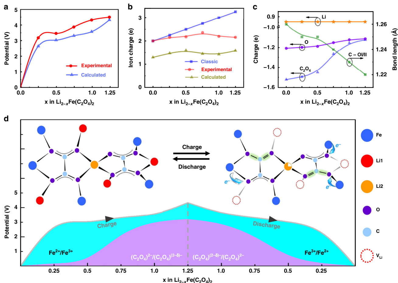
Fig. 4 Computational investigation. a Potential, (b) iron charges, (c) averaged charges for Li, O and C_2O_4 group and calculated mean bond length of C-OI and C-OII versus Li-content in LFOx. d Schematic illustration of iron and oxalate redox mechanism and their contribution to specific capacity in the stabilized charging and discharging process
