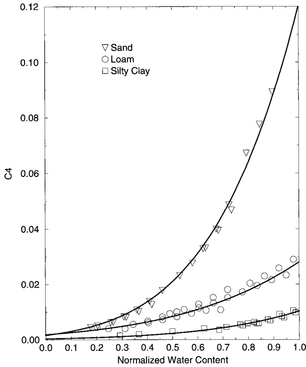
FIG. 3. The C_4 dimensionless coefficient as a function of the interfacial volumetric water content, \bar{w}_{2,3} , for sand, loam, and silty clay soil textures. The interfacial water content has been normalized for each soil texture: the minimum value along the abscissa represents the wilting point, and unity represents the field capacity. The total soil depth d_3 is 2 m, and the root zone depth d_2 is 1 m. Symbols represent results calculated from MLSM using Eqs. (17) and (18). The fits using Eqs. (17) and (19) are shown as solid lines. The corresponding fit coefficients are shown in Table 1.
