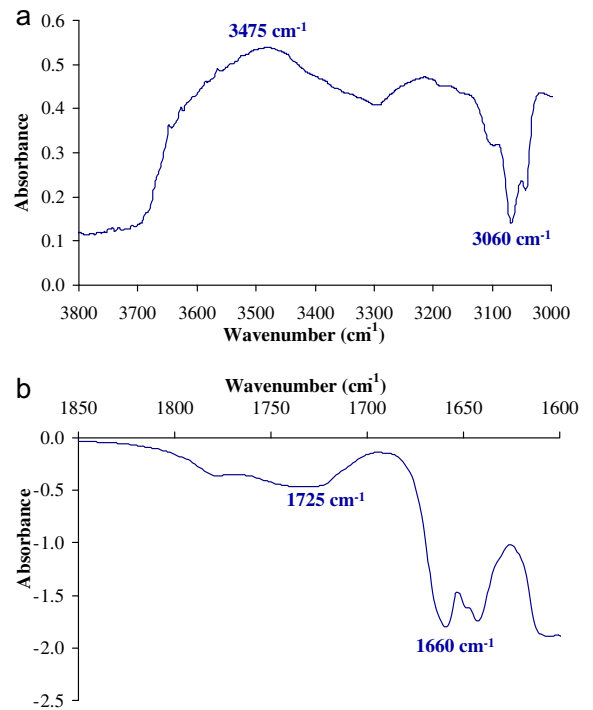
Fig. 4. Effect of \text{NH}_3 treatment on the IR spectrum of 30.7\text{ MGy} irradiated sample (subtracted spectra between treated and untreated sample) in the hydroxyl region (a) and in the carbonyl region (b).
