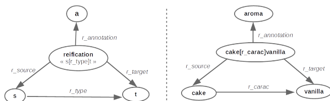
Figure 1: MLSN: relationship annotation scheme.
