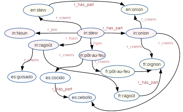
Fig. 1. Pivoted MLSN architecture. in precedes interlingual terms.
