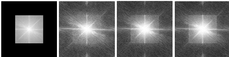
Figure 22: Spectrums of Image I_1 , \bar{I}_1 , \check{I}_1 and \check{\check{I}}_1 . We can see that the spectrums of \check{I}_1 and \check{\check{I}}_1 remain more condensed in the central square than the one of \bar{I}_1 .
