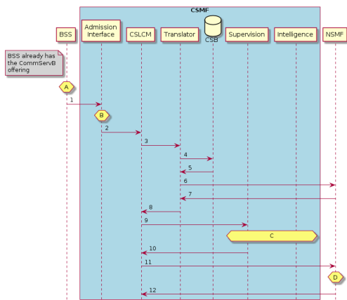
Fig. 4. Sequence diagram for usage (1): new communication service.
