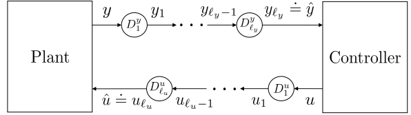
Fig. 4. NCS closed over a WH network with \ell_y field devices in the y -path and \ell_u field devices in the u -path.
