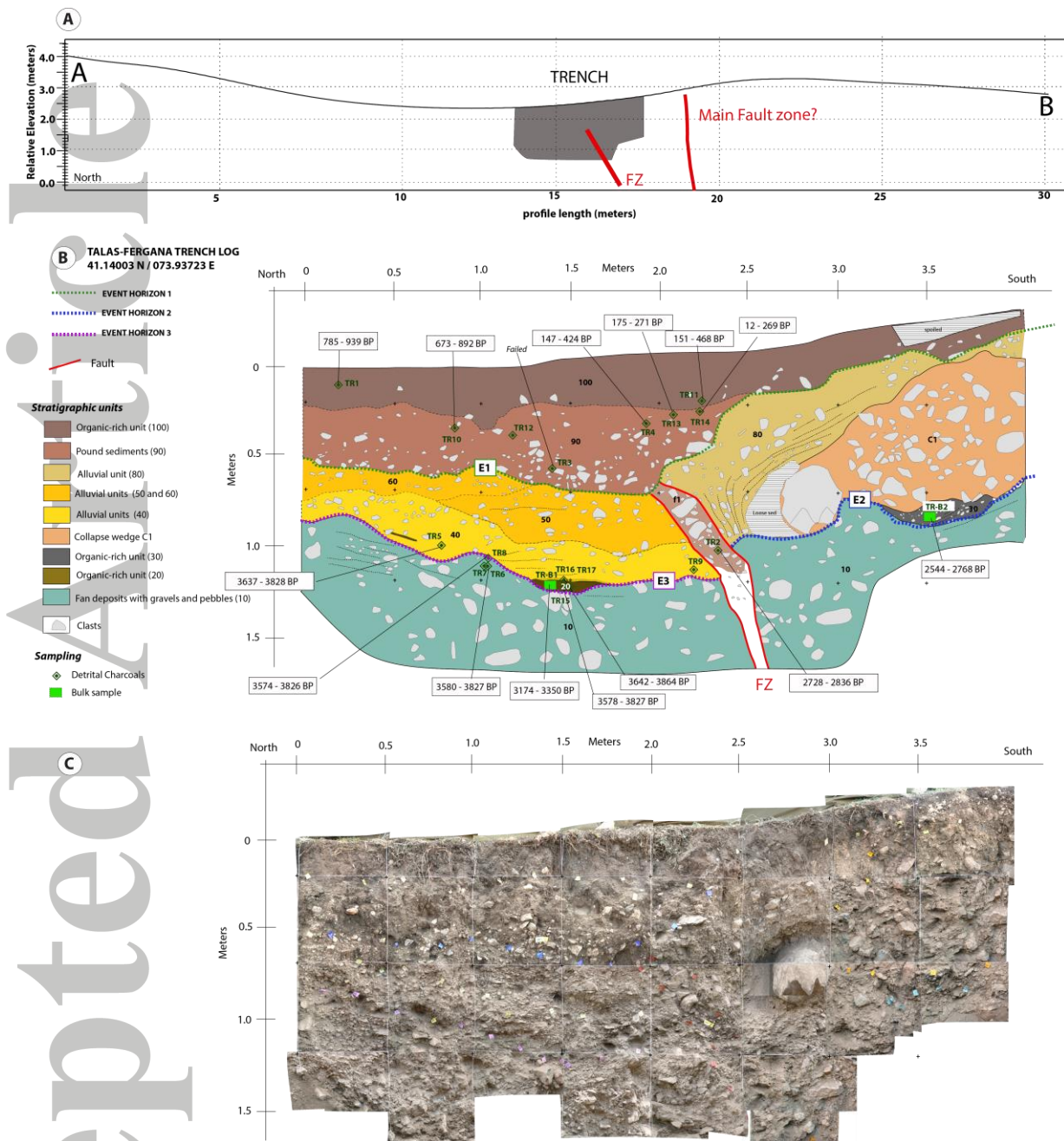
Figure 10: Paleoseismic investigation at the Kyldau site. A) Topographic profile across the fault scarp (see location on Figure 5C). The position of the trench is represented in gray, faults are represented by thick red lines. B) Log interpretation (see text in section 4 for details) with positions of detrital charcoals collected in the trench. The reported ages are calibrated using Intcal13 curves (Reimer et al., 2013). C) Ortho-photo mosaic of the trench.
