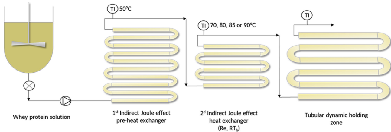
Fig. 2. Schematic representation of the heat treatment pilot.
