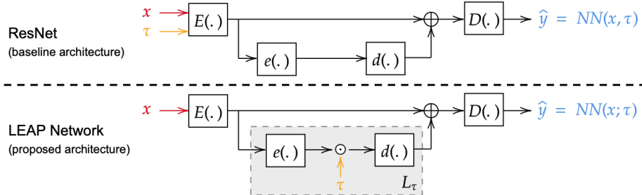
Fig. 2: Baseline and LEAP architectures: Top: ResNet [4] architecture, with \tau as input. Bottom: Proposed LEAP net: \tau intervenes in the latent embedding space. The effect is to make a “leap” in latent space.
