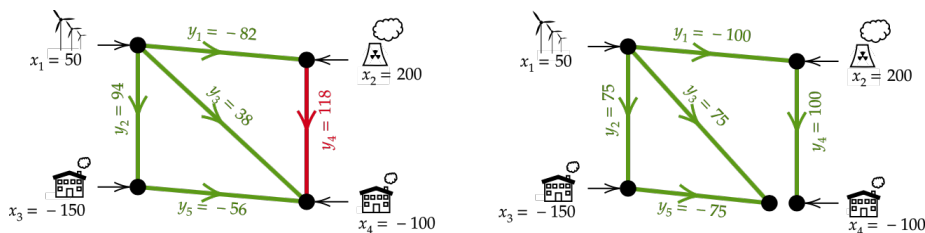
Fig. 1: Electricity is transported from production nodes (top) to consumption nodes (bottom), through lines (green and red edges) connected at substations (black circles), forming a transmission grid of a given topology \tau . Injections \mathbf{x} = (x_1, x_2, x_3, x_4) (production or consumption) add up to zero. Grid operators (a.k.a. dispatchers ) should maintain current flows \mathbf{y} = S(\mathbf{x}, \tau) below thermal limits. Left: Line y_4 goes over its thermal limit 100. Right: A change in topology (splitting of node 6) brings y_4 back to its thermal limit.
