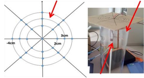
H-field probe
