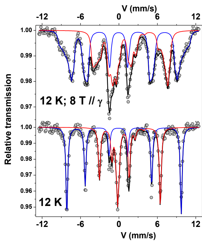
Figure 4. ^{57}\text{Fe} Mössbauer spectra of \text{Fe}_2\text{F}_5(\text{Htaz}) at 12 K in (bottom) zero field and (top) an applied field of 8 T. The blue and red lines correspond to \text{Fe}^{3+} and \text{Fe}^{2+} magnetic components, respectively.
