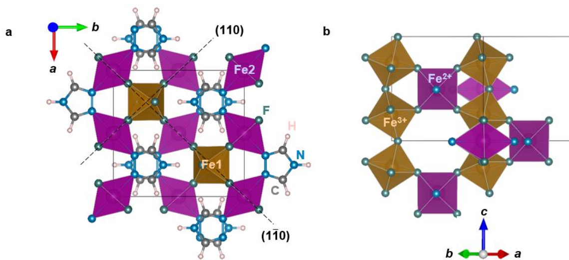
Figure 1. (a) A projection of the refined Im2 structure of \text{Fe}_2\text{F}_5(\text{Htaz}) showing the nearly orthogonal HTB layers in the (110) and (1\bar{1}0) type planes (b) that contain a triangular network of \text{Fe}^{3+} (site 4b ) and \text{Fe}^{2+} (site 4a ) cations connected via fluoride anions.
