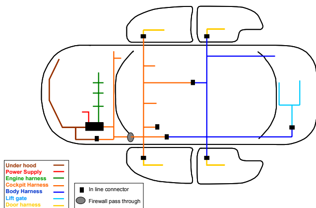
Figure 9: Example of multipiece loom harness
