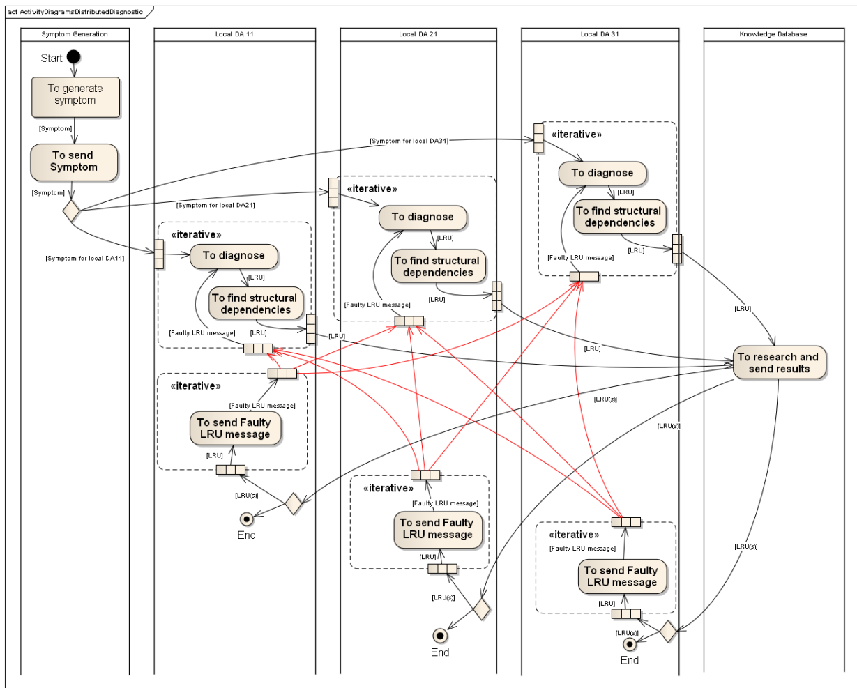
Figure 5: Activity Diagram of the distributed diagnosis system
