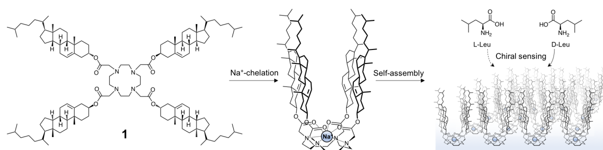
Figure 2. Structure of the cholesterol-armed cyclen designed by Michinobu, Tsukube and co-workers. Formation of its octadentate Na + complex and subsequent self-assembly to chiral host monolayer (at the interface air-water) for mechanical control of enantioselectivity of amino acid recognition.
