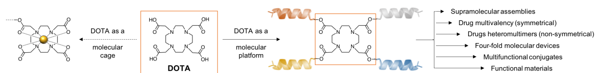
Figure 1. Schematic representation of the uses of DOTA either as molecular cage for chelating metals (left panel) or as platform to assemble multivalent molecular tools (right panel), which is the key topic of the review.
