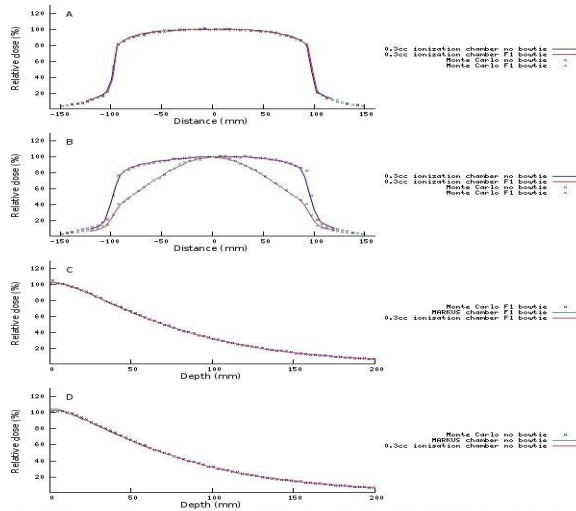
Fig. 1. Comparisons between measurements and MC calculations at 120 kV for the S20 collimator. In-line (Y) and crossline (X) profiles at 1 cm deep are shown in (a) and (b), respectively. Depth dose curves with and without bowtie are shown in (c) and (d), respectively.
