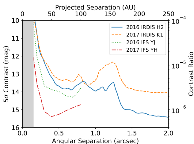
Fig. 3. 5\sigma detection limits for the two SPHERE datasets, after processing using the TLOCI algorithm. The grey shaded region indicates the separations partially or fully blocked by the coronagraph.
