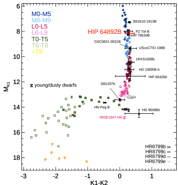
Fig. 9. A colour-magnitude diagram comparing the K1 absolute magnitudes and K1-K2 colours of a range of low-mass stellar and substellar objects from the literature. Synthetic K1 and K2 fluxes were computed for each target from published spectra. A number of young and dusty companions observed with SPHERE or with published K band spectra were added to the diagram. HIP 64892B falls in a similar location to PZ Tel B and HIP 78530B, both young brown dwarfs with late-M spectral types.
