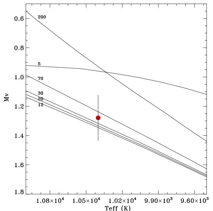
Fig. 1. The V-band absolute magnitude and effective temperature of HIP 64892 compared to predictions from the 5, 12, 20, 30, 70 and 200 Myr isochrones of Bressan et al. (2012). The placement of HIP 64892 is consistent with the estimated local age of 16 Myr within the measured uncertainties.
