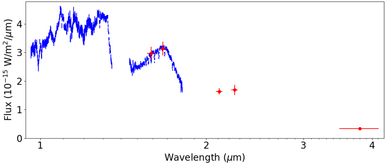
Fig. 6. The observed spectrum of HIP 64892B. SPHERE IRDIS LSS data are shown in blue, while the SPHERE IRDIS and NACO photometric measurements are in red. The errorbars on the x-axis of the photometric measurements represent the FWHM of the filter used.
