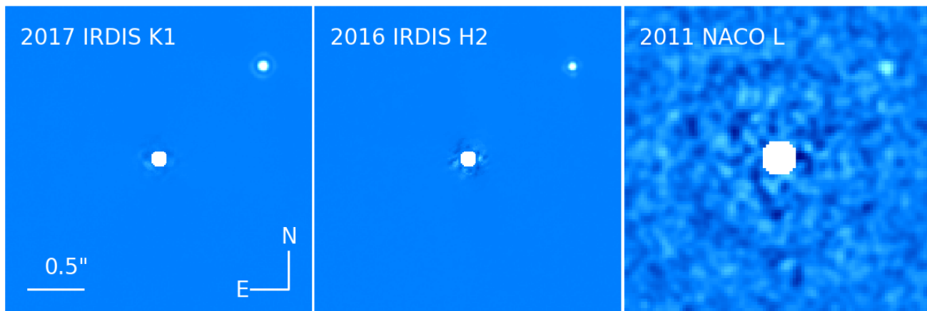
Fig. 2. ADI-processed images from the two SPHERE-IRDIS datasets taken with the K1 and H2 filters, and the NACO data taken with the L' filter. The companion is detected with SNR > 1000 in the two SPHERE epochs, and SNR > 8 in the NACO data.
