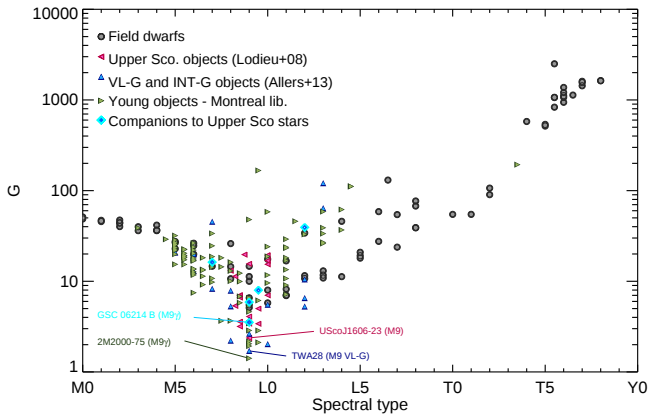
Fig. 7. The G goodness-of-fit statistic plotted as a function of spectral type for a number of objects in the range M0-T8. A clear G minimum is seen at late M spectral types and the best matches are given by young, low surface gravity objects with spectral types of M9.
