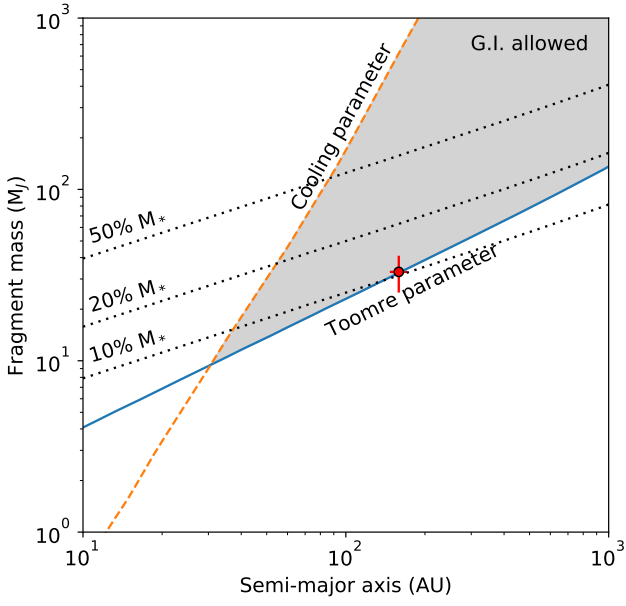
Fig. B.1. Predictions for the fragment masses compatible with production via gravitational instability for HIP 64892. Fragments with masses above the orange dashed line cannot cool efficiently enough, while those below the blue solid line do not satisfy the Toomre criterion. The mass and projected separation of HIP 64892B are marked. We find that HIP 64892B is compatible with in-situ formation via gravitational instability, although further constraints on the semi-major axis are needed to confirm this idea. The initial disk masses required to form fragments of a given size are shown with black dotted lines.
