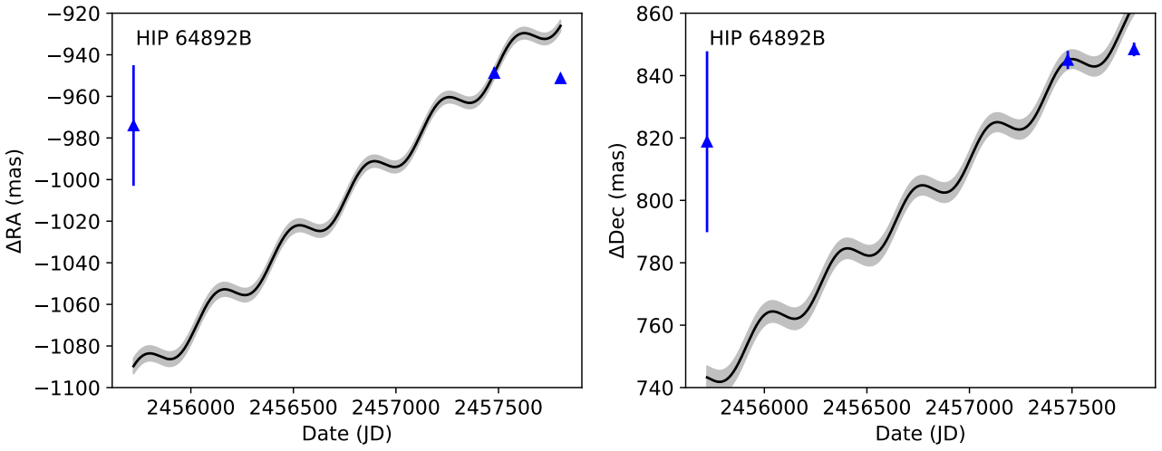
Fig. 4. The measured position of HIP 64892B relative to HIP 64892A. The 2011 NACO L', 2016 IRDIS H2 and 2017 IRDIS K1 positions are shown with blue triangles. The predicted motion for a stationary background object relative to the 2016 position is marked by the black line, with its uncertainty represented by the grey shaded region. The observed positions of HIP 64892B strongly conflict with the predictions for a background object, suggesting that it is co-moving.
