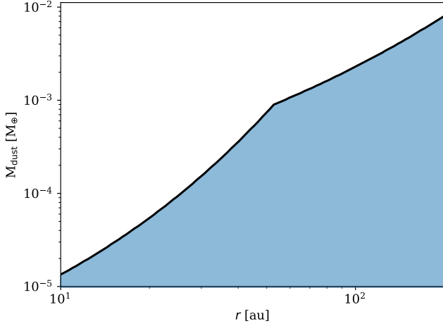
Fig. A.1. The blue-shaded area shows the region in the r - M_{\text{dust}} plane, in which a debris disk could be present and remain compatible with the mid- and far-IR observations.
