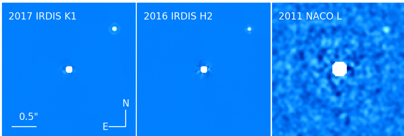
Fig. 2. ADI-processed images from the two SPHERE-IRDIS datasets taken with the K1 and H2 filters, and the NACO data taken with the L' filter. The companion is detected with \text{SNR} > 1000 in the two SPHERE epochs, and \text{SNR} > 8 in the NACO data.
