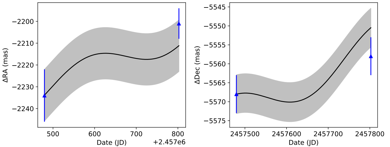
Fig. 5. Same as Fig. 4, showing the measured position of companion candidate 1 with respect to HIP 64892A. This object agrees with the prediction for a background object.
