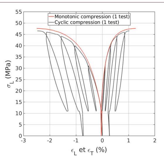
Figure 5: Comparison between the cyclic compressive test and the corresponding monotonic test under a 10 MPa pressure. Longitudinal strains \epsilon_L negative.
