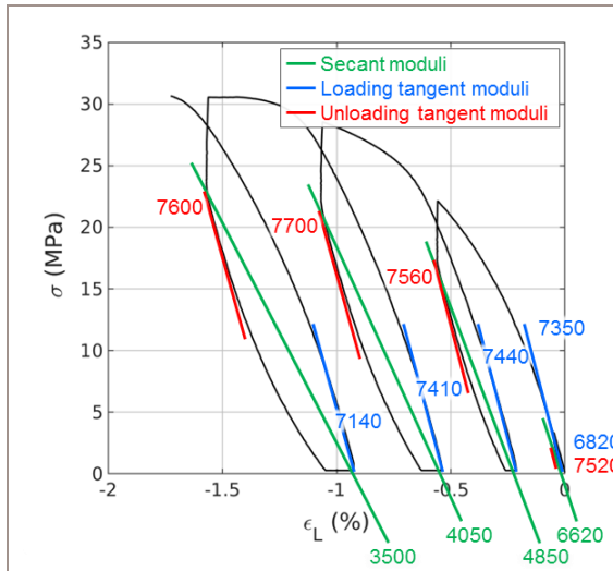
Figure 6: Secant and tangent longitudinal moduli for a no confined compressive test.
