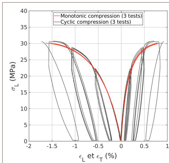
Figure 4: Comparison between the cyclic compressive test and the corresponding monotonic test (no confinement). Longitudinal strains \epsilon_L negative.
