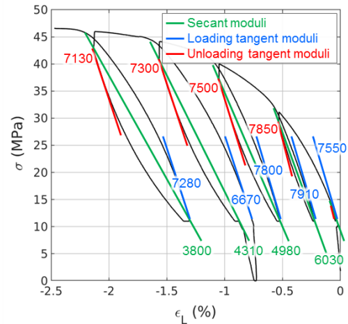
Figure 7: Secant and tangent longitudinal moduli for a confined (10 MPa) compressive test.
