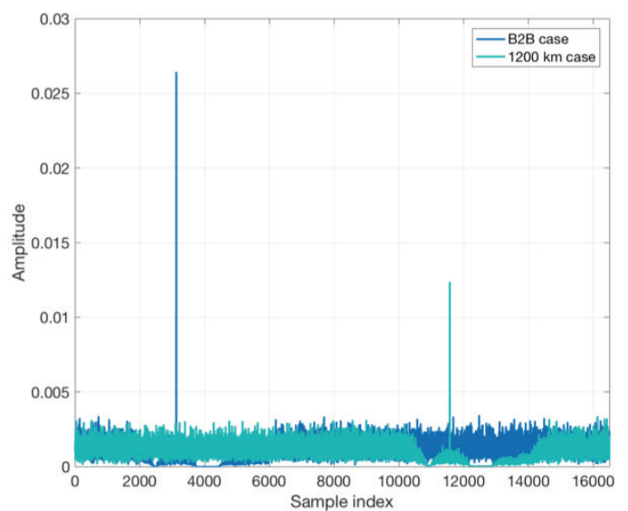
Fig. 4. Cross-correlation functions of the frame synchronization in the back-to-back configuration and after 1200 km transmission. The SoF corresponds to the peak maxima.
