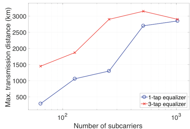
Fig. 9. Maximum transmission distance versus number of subcarriers subjected to 1-dB OSNR penalty at a BER of 3.8 \times 10^{-3} using 1-tap and 3-tap equalizers for CD compensation.
