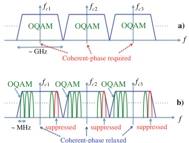
Fig. 1. Examples of multiple sub-channels multiplexing in WDM systems. a) Coherent-phase lasers required; b) Coherent-phase lasers relaxed with a negligible guard band.
