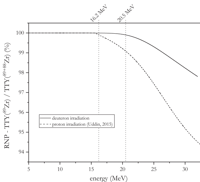
Fig. 6. Radionuclidic purity at the end of an instantaneous bombardment.
