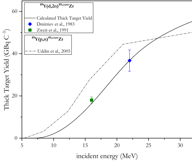
Fig. 2. Thick Target Yield for ^{89}\text{Y}(d,2n)^{89}\text{Zr} nuclear reactions compared with TTY obtained from (p,n) reaction [27].
