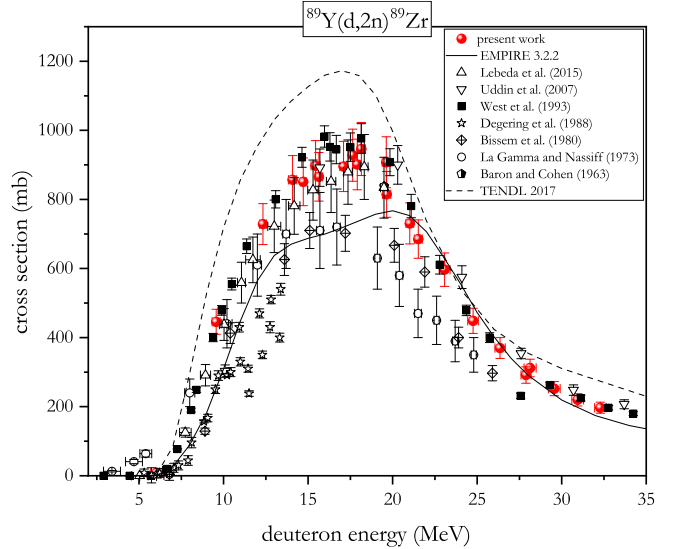
Fig. 1. Excitation functions for ^{89}\text{Y}(d,2n)^{89}\text{Zr} nuclear reactions.
