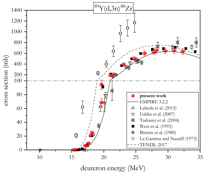
Fig. 3. Excitation functions for ^{89}\text{Y}(d,3n)^{88}\text{Zr} nuclear reactions.
