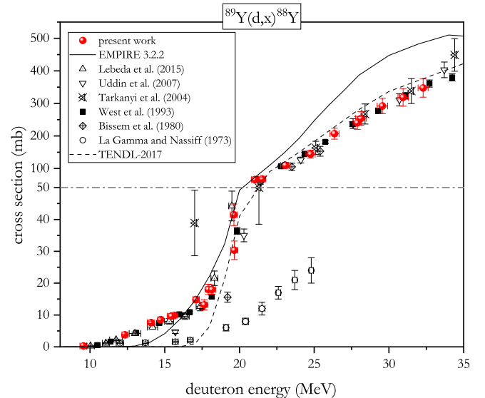
Fig. 5. Excitation functions for ^{89}\text{Y}(d,x)^{88}\text{Y} nuclear reactions.
