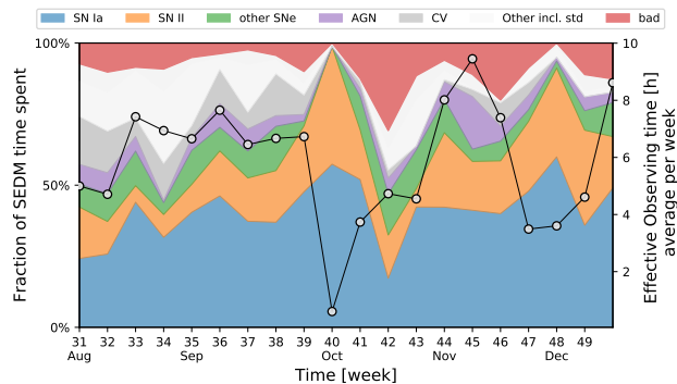
Fig. 15. Use of the SEDM time since PYSEDM is the sole SEDM pipeline (early August 2018) and until redaction of this paper (19 weeks). Color bands show the fraction of target observed per week sorted by type (see legend); left axis. The running line with gray markers shows the evolution of the effective time spent on target per night (weekly average): right axis.
