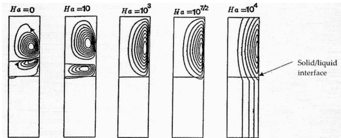
Figure 3: Illustration of the enthalpy-porosity based computations : effect of constant magnetic field ( 0 \leq Ha = (\sigma BL^2/\mu)^{1/2} \leq 10^4 ) opposite to gravity on multicellular flow corresponding to Ra_T = 10^7 for vertical Bridgman configuration [El Ganaoui, 2002].
