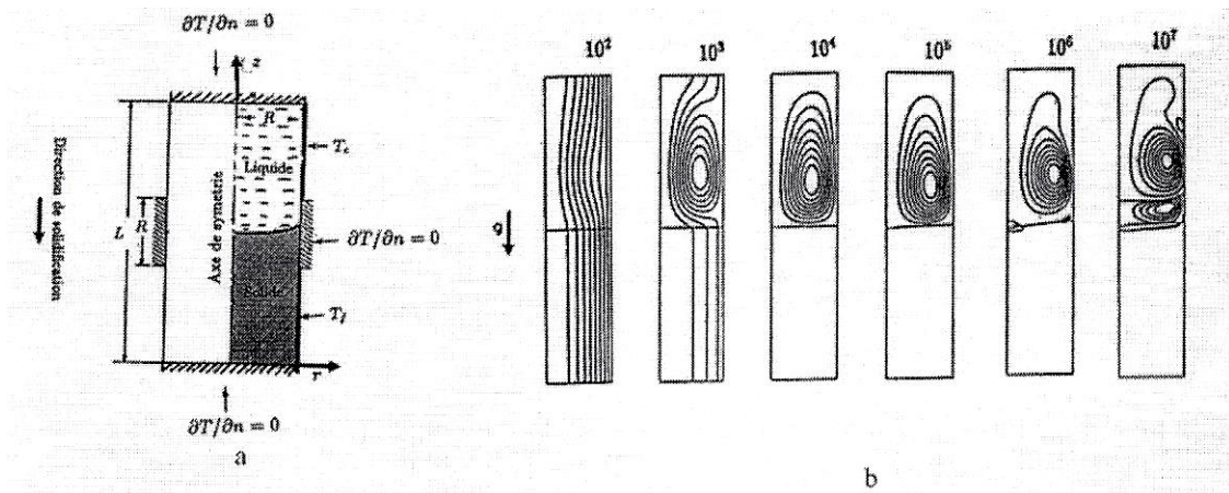
Figure 2: illustration of the enthalpy-porosity based computations: melt under directional solidification using vertical Bridgman method (a) for 10^2 \leq Ra_T = g\beta(T_h - T_c)L^3/\nu\alpha \leq 10^7 (i.e gravity effect) showing evolution from monocellular to multicellular flow (b) Simulation corresponding to an enthalpy porosity formulation/Finite Volumes method [El Ganaoui, 2002].
