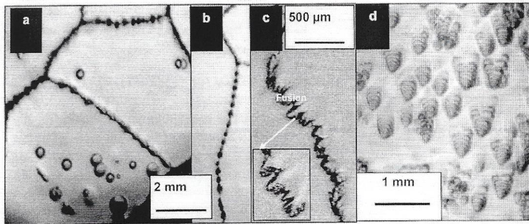
Figure 6: a) Liquid droplets grain– b), c) Morphological instability at grain boundaries d) Arrays melting dendrites in a grain [Benielli et al, 2002]
