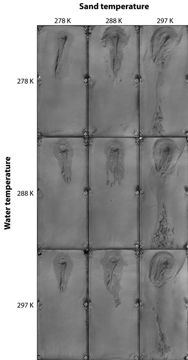
Fig. 4. Mosaic of typical morphological results obtained after the water flowed on the sand test bed as a function of sediment and water temperature. Orthoimages obtained by photogrammetry of the surface. The width of the test bed is about 40 cm. The top of the slope is located at the top of the image. The selected orthoimages correspond to the following runs: S278-W278-1; S288-W278-2; S297-W278-2; S278-W288-3; S288-W288-3; S297-W288-1; S278-W297-3; S288-W297-3; S297-W297-3 (from left to right and top to bottom).
