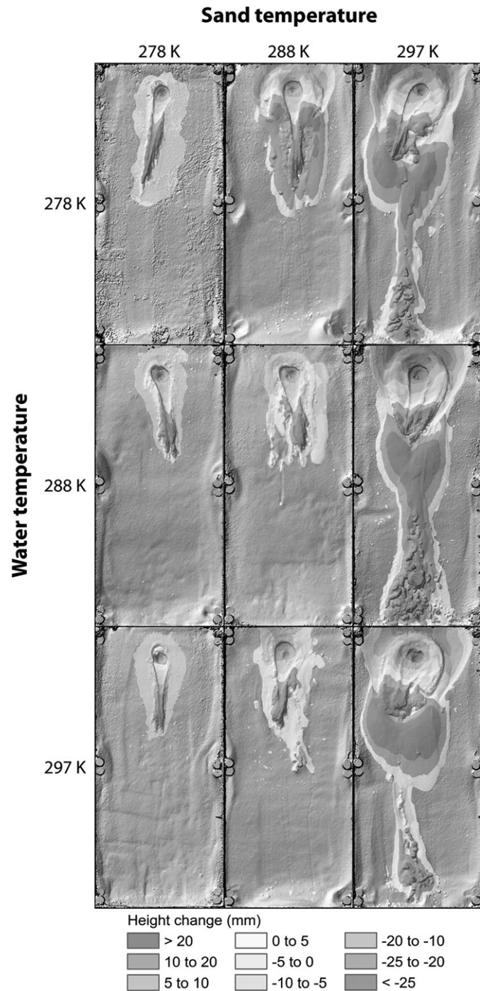
Fig. 12. Mosaic of the elevation difference between start and end of experiments as a function of sediment and water temperature. The elevation differences are overlain onto a hillshade relief model derived from the DEMs (1 mm/pix) obtained by photogrammetry. The width of the test bed is about 40 cm. The top of the slope is located at the top of the image. S278-W278-1; S288-W278-2; S297-W278-2; S278-W288-3; S288-W288-3; S297-W288-1; S278-W297-3; S288-W297-3; S297-W297-3 (from left to right and top to bottom).
