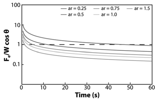
Fig. 19. Evolution of the ratio of the lifting force F_c to the weight force W \cos \theta of a block over a slope of 25^\circ . The ratio is calculated for different aspect ratios (ar) D/H of pellets for a surface temperature of T_0 = 297 K and D = 2 cm in the Mars Simulation Chamber. The physical parameters of our experiments in the Mars Simulation Chamber can be found in Raack et al. (2017). Levitation occurs when the ratio F_c/W \cos \theta is greater than 1 (dashed black line).
