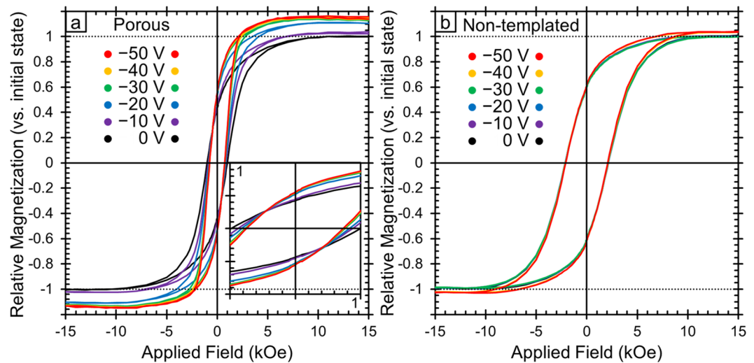
Figure 7. Room temperature magnetic hysteresis loops for both the porous (a) and non-templated (b) films as a function of applied voltage. In this case, the voltage was applied for 20 min and then the hysteresis loop was measured for 20 min leading to a total time of 40 min between each loop. To compare between the samples, the saturation magnetization ( M_S ) was normalized such that the initial state (0 V) was set to 1. The inset in panel a shows the region near zero applied field in order to better observe the changes in coercivity.
