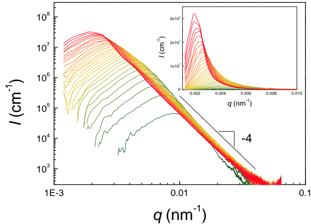
FIG. 6. Time evolution of the scattered intensity for a sample with Glu = 44\% following a temperature quench of depth \Delta T = 7^\circ\text{C} . The time elapsed since the quenched temperature has been reached varies from 1 to 300 s, when the color gradually changes from green to red.
