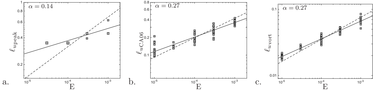
Figure 3. Evolution of the typical length scales of the flow as a function of the Ekman number, same representation as in figure 2, but for numerical dynamo in the multipolar-fluctuating state.
