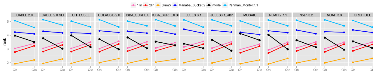
FIG. 2. Ranks of LSMs relative to benchmarks, averaged over all metrics and sites [after Fig. 4 in Best et al. (2015)]. Each column shows a different LSM. Within each column, sensible heat (i.e., Q_h ) and latent heat (i.e., Q_{le} ) are shown. The LSM is in black, and various benchmarks are shown in comparison. The vertical axis shows the average performance rank for each model under four metrics over the 20 FLUXNET site datasets. In each case, a lower value indicates better relative performance. The 3km27 model clearly outperforms the LSMs for both variables, and the two linear regressions consistently outperform all LSMs for sensible heat.
