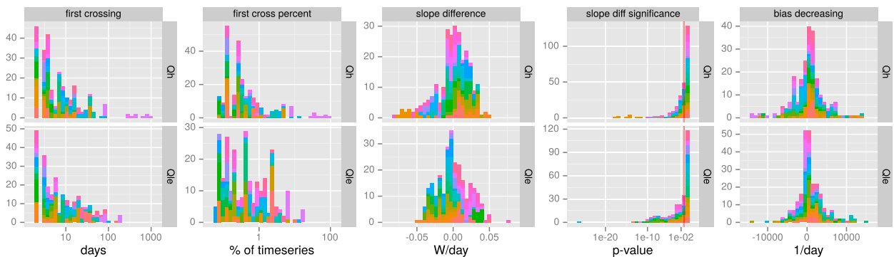
FIG. 7. Histograms of model spinup metrics, based on daily averages, from all LSMs at all sites. From left to right: day at which the simulated series crosses the observed series; day at which the simulated series crosses the observed series, but as a percentage of the time series; difference in the slopes of linear regressions of simulated and observed series over time ( W \text{ day}^{-1} ); significance of the difference in the previous metric (values left of the red line are significant at the \alpha = 0.05 level; \sim 44\% of all values); and the rate at which the bias is decreasing, measured by mean(error)/slope(error) (negative values indicate the simulations have a trend toward the observations). Colors indicate the FLUXNET site at which the simulation is run.
