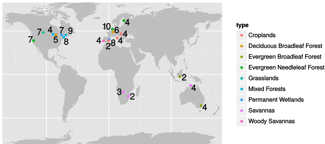
FIG. 1. The locations of the 20 flux tower sites in the PLUMBER experiment. The IGBP vegetation type is represented by color and the numbers indicate the years of data used in the PLUMBER experiment. Site data are given in Table 1.
