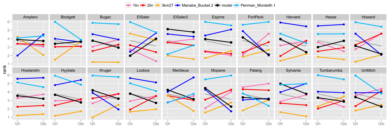
FIG. 5. As in Fig. 2, but for results where each cell represents the average rank of all LSMs at each individual FLUXNET site. The gray line is identical to that shown in Fig. 4.
