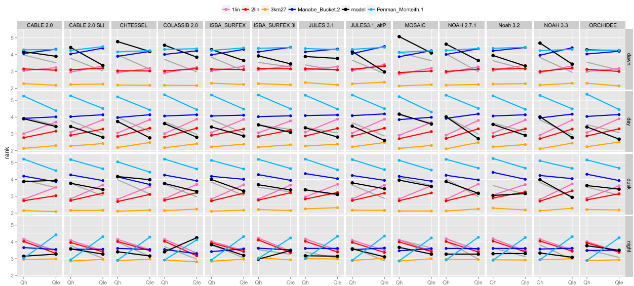
FIG. 11. As in Fig. 2, but for results split by daily cycle. The four rows represent the 6-h periods around dawn (0300–0900 LT), noon (0900–1500 LT), dusk (1500–2100 LT), and midnight (2100–0300 LT). The gray line is identical to that shown in Fig. 4.
