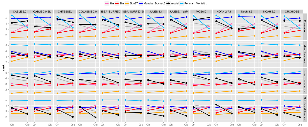
FIG. 4. As in Fig. 2, but for results where each row represents an individual metric (see Table 3 for metric definitions). The gray line shows the original LSM mean rank for comparison (as in Fig. 2, though note that these data are only comparable with the black line, and not the benchmarks that have also changed).
