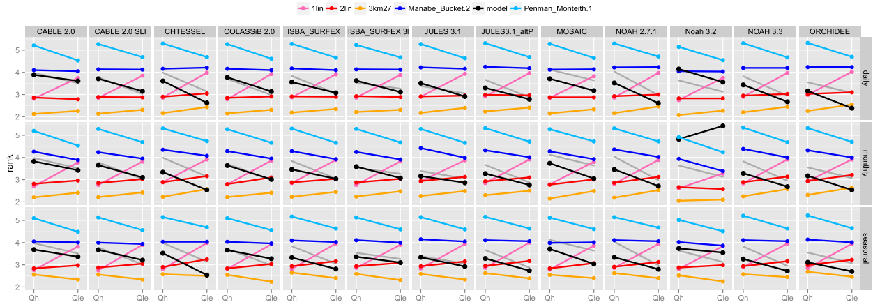
FIG. 6. As in Fig. 2, but for values that are averaged over daily, monthly, and seasonal time periods. The gray line is identical to that shown in Fig. 4.
