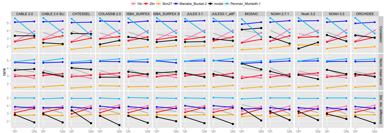
FIG. 10. As in Fig. 2, but for high-frequency response only, by metric; LSMs are bias corrected on a daily basis and then have the daily cycle in the errors removed. The gray line is identical to that shown in Fig. 4. The mean bias error metric is not included because it is trivially zero because of the bias correction process.
