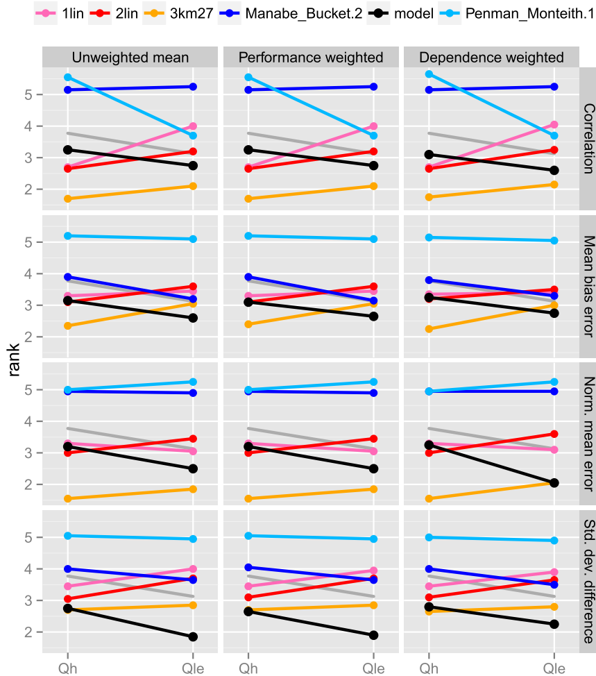
FIG. 12. As in Fig. 2, but for the results for three different means across all LSMs, by metric. The gray line is identical to that shown in Fig. 4. In general, we should expect means to perform better under all metrics except the standard deviation metric, as the averaging process acts as a smoother, removing noncorrelated noise from the model results.
