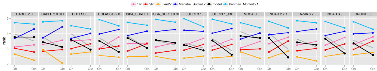
FIG. 8. As in Fig. 2, but for energy conservation constrained empirical models. The gray line is identical to that shown in Fig. 4.
