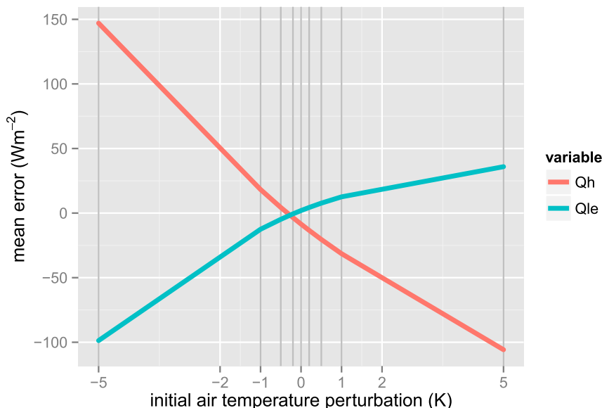
FIG. 13. Mean error in Q_h and Q_{le} as a result of perturbing the initial canopy air temperature at each time step, in CABLE at the Tumbarumba site in southeastern Australia. Temperature was perturbed by \pm(5, 2, 1, 0.5, 0.2) K, and a control run is included. All model parameters were left as default values. The response in Q_h to negative temperature perturbations is about 50% stronger than in Q_{le} , and about 3 times stronger for positive perturbations.
