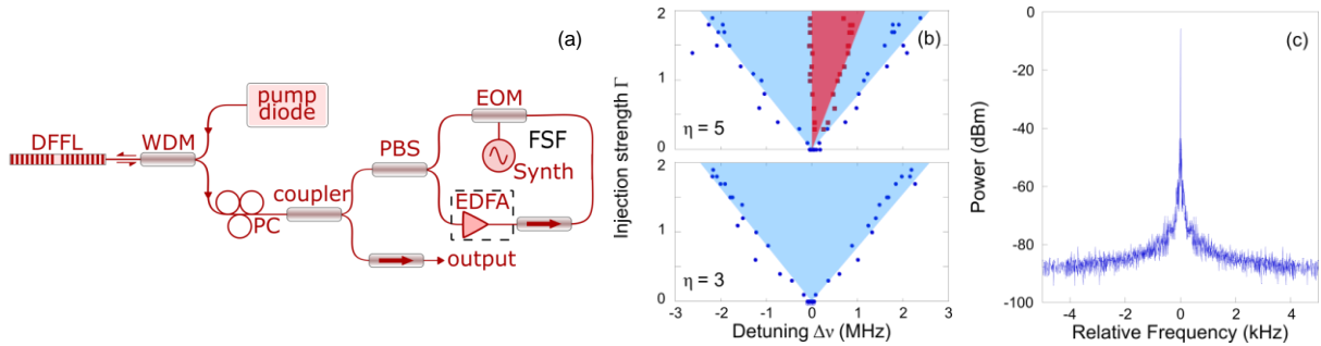
Fig. 1 (a) Experimental scheme. The optional EDFA permits here to control the re-injected power. (b) Normalized injection strength \Gamma with respect to the detuning \Delta\nu at two different excitation ratios \eta . Colored areas delimit the different regimes. White: unlocked, blue: locked, red: intensity modulated. (c) RF Spectrum of the locked DFFL beat.
