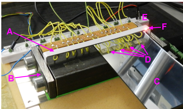
Figure 6: Picture of the experiment: A) Staple shaped aluminum beam, the velocity is controlled within a rectangular region on the upper part; B) Fixture of the beam to realize clamp-clamp boundary conditions; C) Mirror showing the ceramics; D) Reflection revealing some of the ceramics fixed beneath the beam. The second ceramic from the left is split as explained in the text; E) Electrical connections of transducers allowing the reconfiguration according to the set of ceramics used; F) Laser spot positioned at one of the corner of the studied region.
