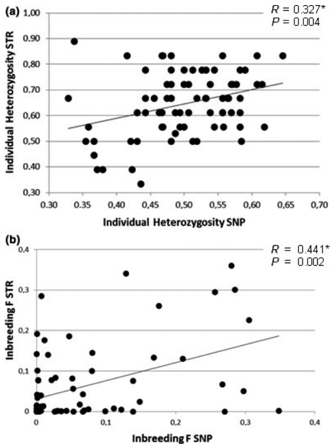
FIGURE 3 Correlation between SNPs and STRs markers ( N = 76 individuals) for (a) individual heterozygosity by loci (calculated in GenAEx) and (b) inbreeding F (calculated in COANCESTRY).
