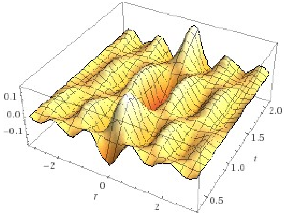
FIGURE 3. Approximate Analytical Solution in (59) for \beta = 0.50
