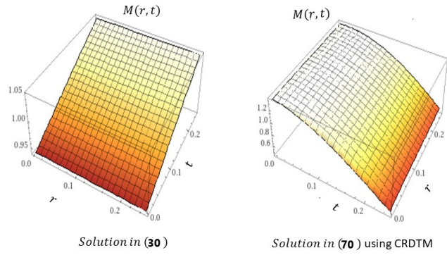
FIGURE 7. Comparison of Solutions in (30) and (70) for \beta = 1
