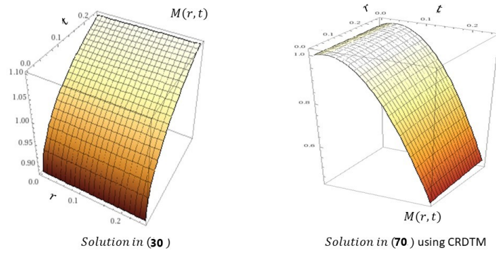
FIGURE 8. Comparison of Solutions in (30) and (70) for \beta = 0.75
