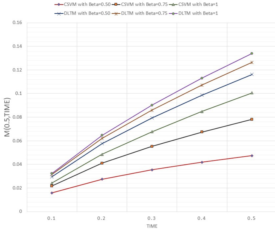
FIGURE 4. Comparison of Analytical and Approximate Solutions in (73) and (72) for different values of \beta at a fixed r = 0.5
