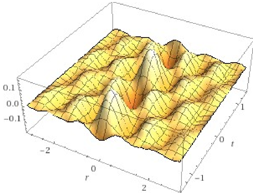
FIGURE 1. Approximate Analytical Solution in (59) for \beta = 1
