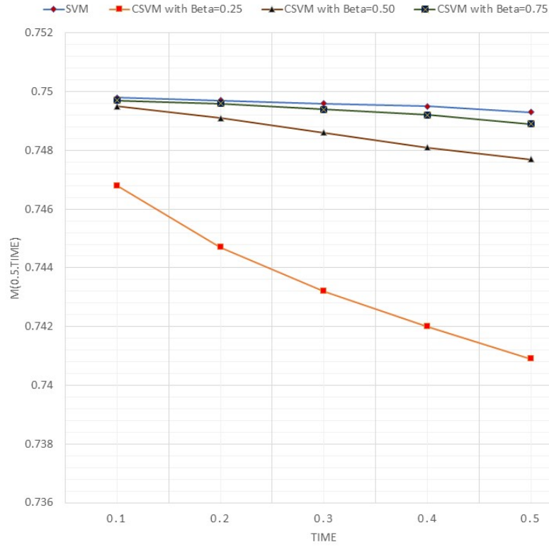
FIGURE 4. Comparison of Analytical and Approximate Solutions in (73) and (72) for different values of \beta at a fixed r = 0.5
