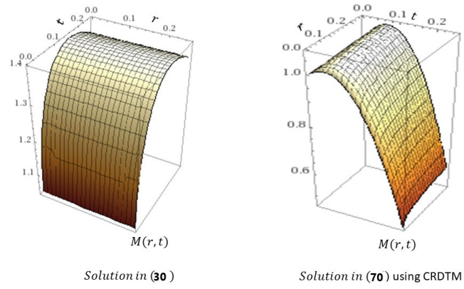
FIGURE 9. Comparison of Solutions in (30) and (70) for \beta = 0.25
