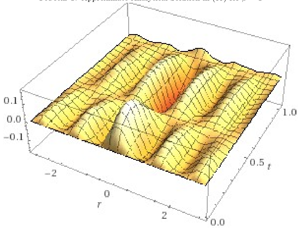
FIGURE 2. Approximate Analytical Solution in (59) for \beta = 0.75
