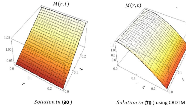
FIGURE 7. Comparison of Solutions in (30) and (70) for \beta = 1
