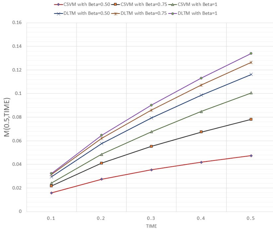
FIGURE 4. Comparison of Analytical and Approximate Solutions in (73) and (72) for different values of \beta at a fixed r = 0.5
