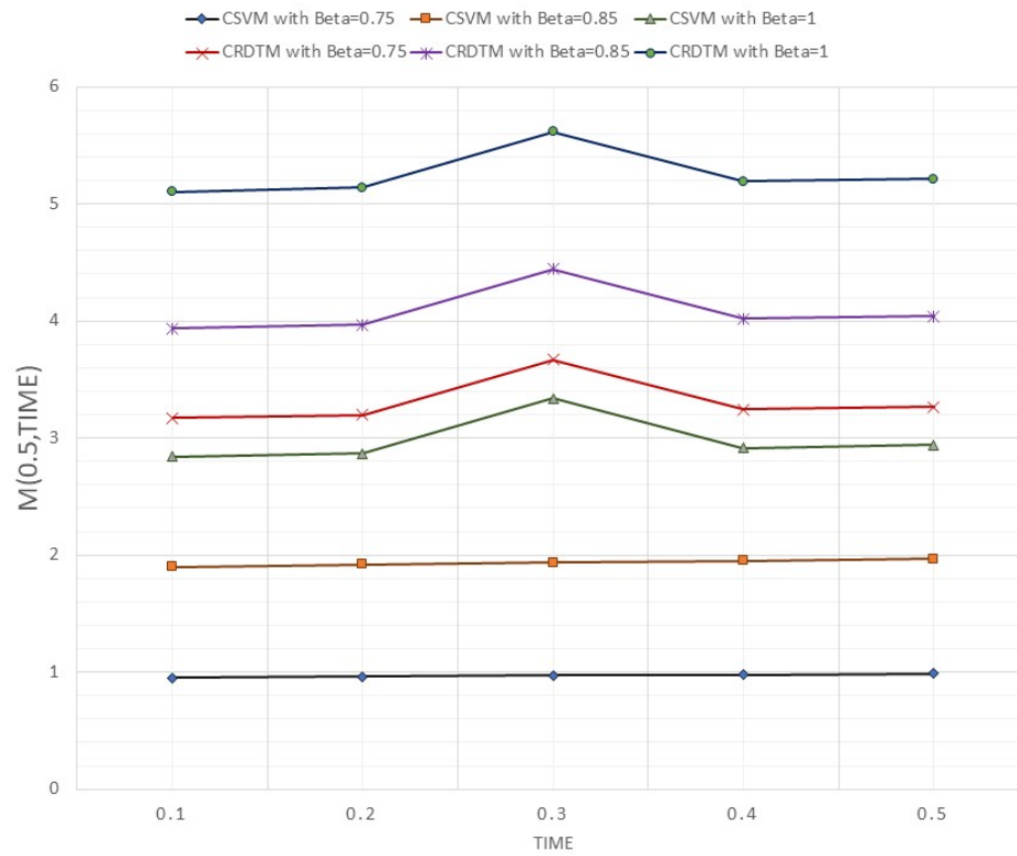
FIGURE 6. Comparison of Approximate Solutions in (84) and (70) for different values of \beta at a fixed r = 0.5
