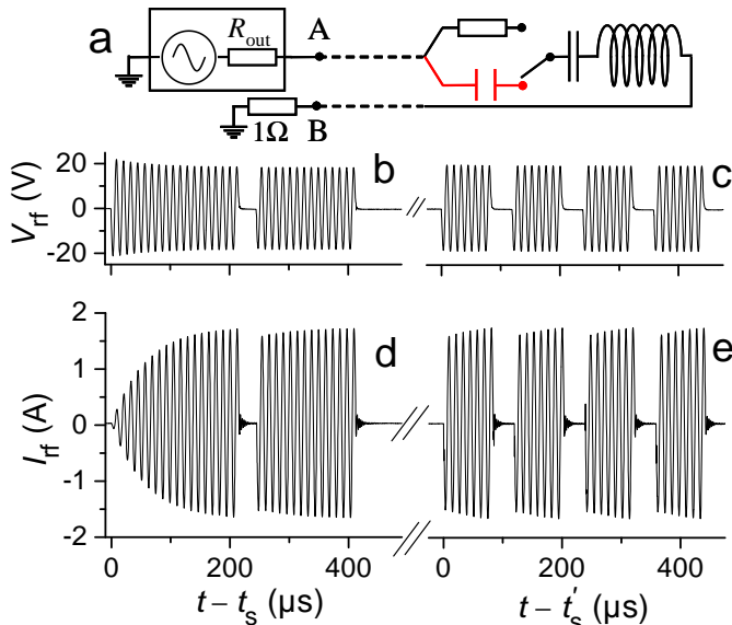
Figure 5: Voltage (panels b and c) and current (d and e) recordings at frequency f_0 in the tuned U coil (circuit diagram a). The switch (with IRF840 MOSFETs) was opened only during the rectangular rf pulses. b,d: a pair of 18- and 14- \tau_0 -long voltage pulses with magnitude V_m = 20 V was used. The gap between the pulses was 2.5- \tau_0 long and the phase of the rf carrier was 180°-shifted for the second pulse, yielding the same start phase \varphi_s = 90^\circ . c,e: a series of 7- \tau_0 -long voltage pulses with the same magnitude and start phase was applied, with 3- \tau_0 -long delays between pulses. The difference t'_s - t_s was 1061- \tau_0 -long ( \approx 12.8 ms) in this example. Energy built up during the first “charging” pulse was efficiently stored in the tuning capacitor between pulses, and more than 90% was recovered every time the switch was opened again with a suitable timing (see text).
