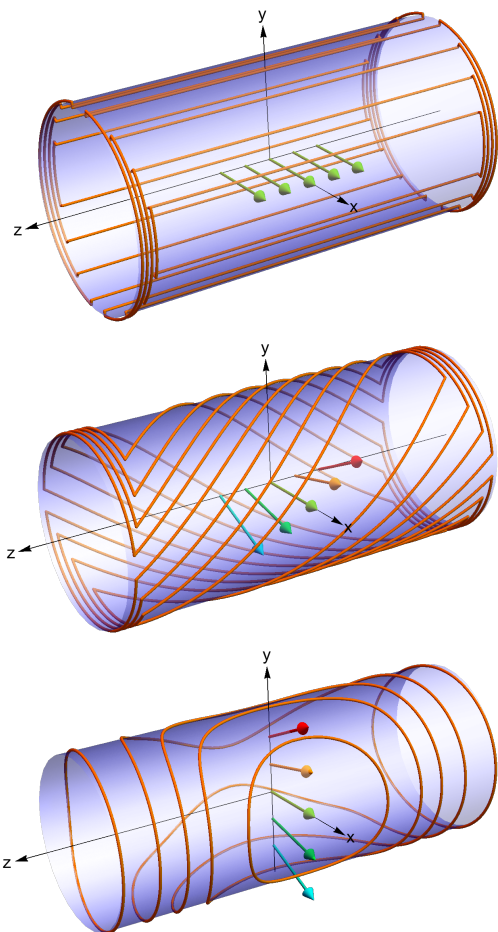
Figure 2: Wire drawings of the U (top), PG Z (middle) and PG Y (bottom) rf coils. All coils were wound with 0.43 mm diameter copper wire on poly(methyl methacrylate) (a.k.a. PMMA or acrylic) tubes of length 290 mm, with outer diameters of 150 mm, 133 mm, 120 mm, respectively. The arrows highlight the nominal field distributions in the central region of each coil, with spatial phase distinguished by color to guide the eye.
