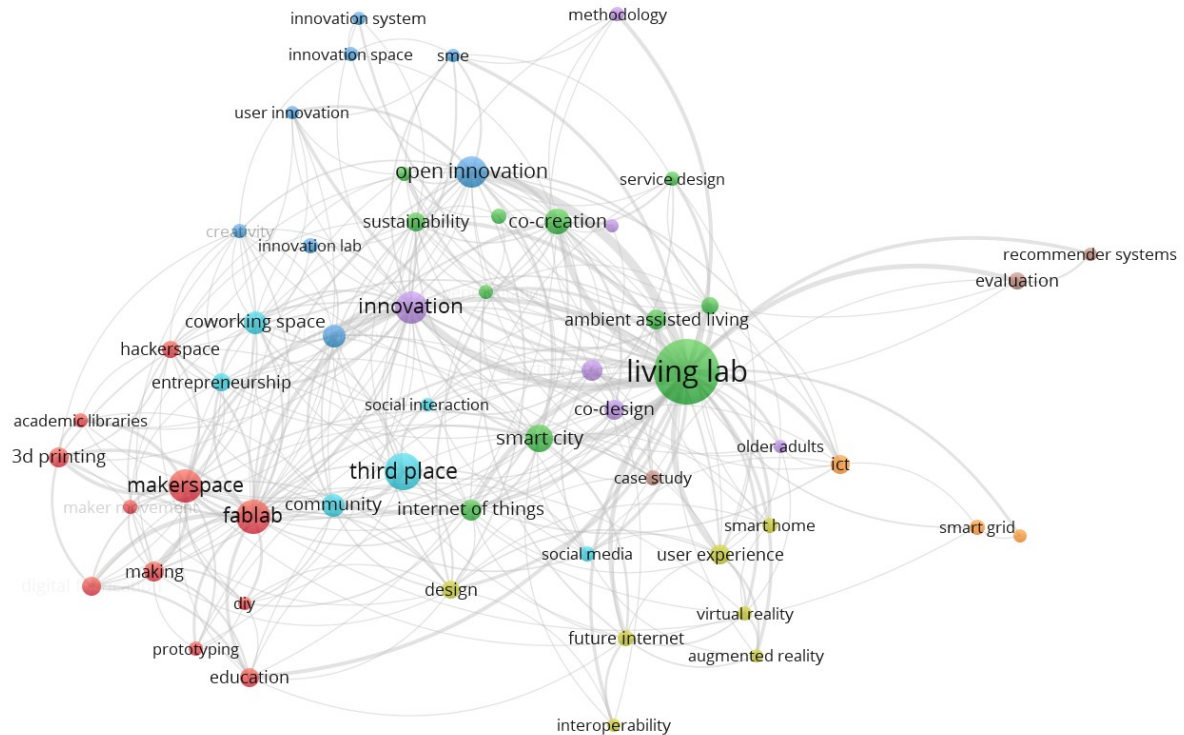
Fig. 3. Network visualization
