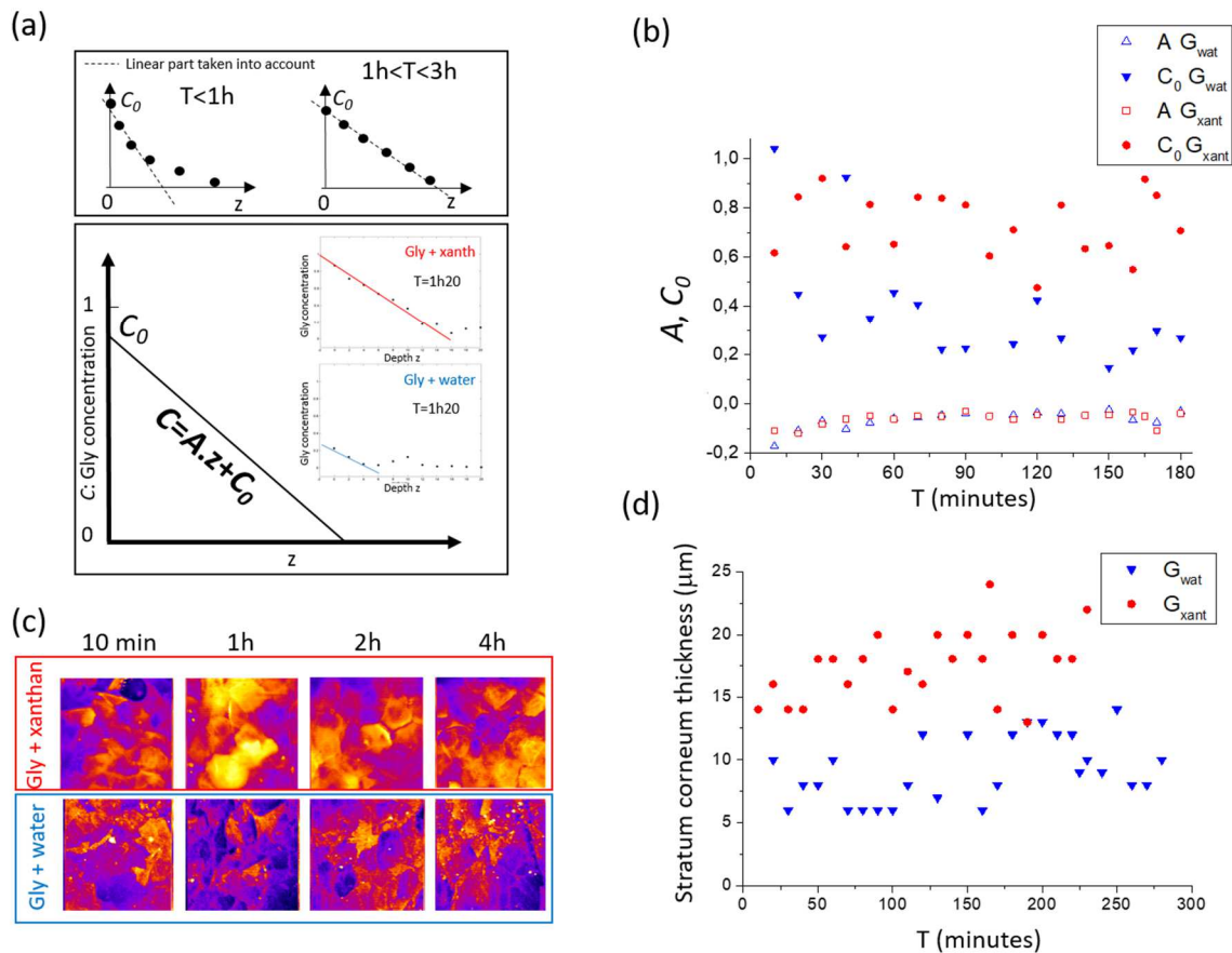
Figure 4: Evolution of deuterated glycerol concentration and stratum corneum (SC) thickness after topical application time T . (a) A linear regression is used to fit concentration profiles with depth for both water and xanthan gel formulations (insets). (b) Evolution of concentration profile slopes A and surface concentration C_0 with time T , highlighting a surface reservoir created by the xanthan gel. (c) SC TPEF images versus T and (d) SC thickness evolution with time T .
