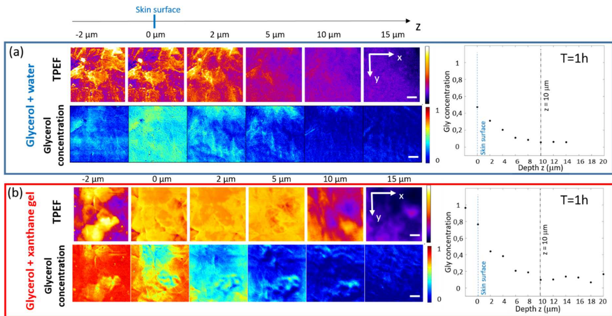
Figure 2: In vivo TPEF and deuterated glycerol concentration in human forearm with increasing depth T=1\text{h} after the application of 30 \mu\text{L} of formulation on the skin surface. Deuterated glycerol is diluted at 40% (mass) into water (formulation G_{\text{wat}} ) (a) and xanthan gel (formulation G_{\text{xant}} ) (b). TPEF images with depth z enable to visualize the corneocytes and to locate the skin surface. The graphs on the right show the in plane ( x,y ) integrated deuterated glycerol concentration with depth z . Xanthan gel retains a glycerol reservoir on the skin surface. Glycerol concentration: 1 corresponds to a concentration of 40% mass.. TPEF images are in arbitrary unit. Scale bar: 20 \mu\text{m}
