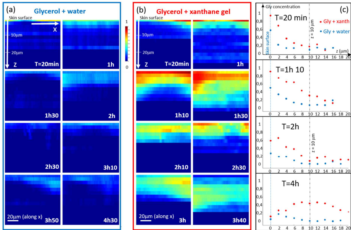
Figure 3: In vivo time lapse glycerol percutaneous penetration after the application at T=0 of 30\ \mu\text{L} of formulation on the skin surface. Deuterated glycerol is diluted at 40% (mass) into water (formulation G_{\text{wat}} ) (a) and xanthan gel (formulation G_{\text{xant}} ) (b). (c) In plane ( x,y ) integrated deuterated glycerol concentration evolution in time for G_{\text{wat}} (blue dots) and G_{\text{xant}} (red dots). Glycerol concentration: 1 corresponds to a concentration of 40%. In (a) and (b) note that scale bars are not the same along x and z axis.
