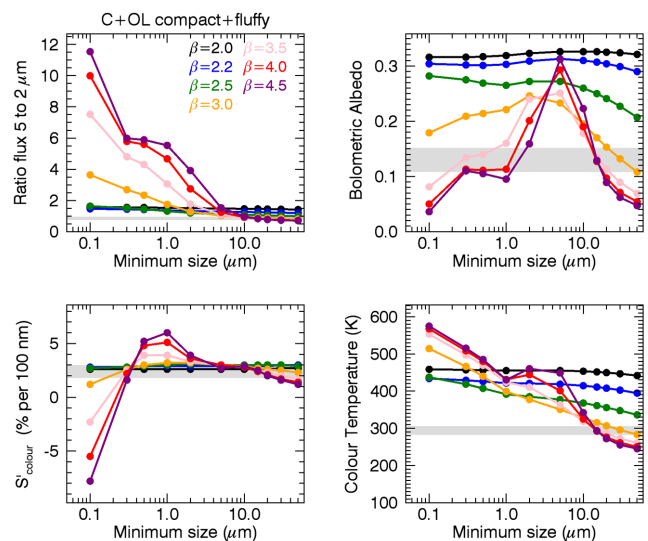
Figure 4. Replaces Fig. 11 of Bockelée-Morvan et al. (2017). Results for relative fractions of 25 per cent of fractal aggregates and 75 per cent of moderately porous carbon/olivine mixtures ( P_{\max} = 0.5 ). The grey area (not included in the original figure) shows the range of observed values on 13 and 14 September 2015 (pre-outburst).
