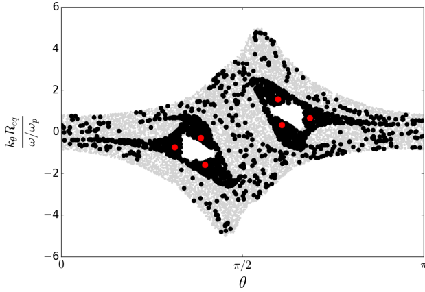
Fig. 18. Snapshot of the evolution of a bundle of trajectories as they intersect the PSS, represented by black dots, at \Omega/\Omega_k = 0.706 . The phase space zones where black dots are dense correspond to regions enclosed by partial barriers. The trajectories are initially in the neighborhood of the two main islands. One of the central periodic orbits of these zones is indicated by colored dots (large gray dots).
