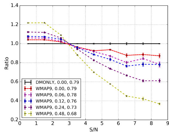
Figure 7. Relative percentage differences in peak counts with respect to the DMONLY peak count distribution (Fig. 6a). For the DGB/SB survey, five models ( M_\nu = 0.00, 0.06, 0.12, 0.24, and 0.48 eV, all with fiducial baryonic physics) of the WMAP 9 cosmology are compared with the DMONLY model in order to determine percentage differences in each interval of S/N. The legend is labelled as Cosmology, M_\nu (eV), and S_8 .
