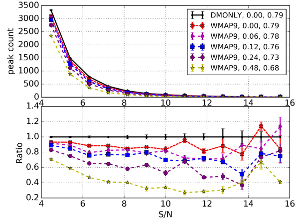
Figure 5. Impact of summed neutrino mass with underlying fiducial baryonic physics ( M_\nu = 0.00, 0.06, 0.12, 0.24, and 0.48 eV models, all with fiducial baryonic physics, see Table 1). The left-hand panel shows the halo mass function (plotted for redshifts out to z = 0.9 ) and the right-hand panel shows the S/N peak count distributions, compared with the DMONLY model (collisionless dynamics). This is shown for the DGB/SB (30 gal arcmin ^{-2} ) survey based on WMAP 9 cosmology. The legend is labelled as Cosmology, M_\nu (eV), and S_8 . The comparisons in the bottom panels are with respect to the DMONLY (collisionless dynamics) model. The error bars show the estimated error using Poisson noise ( \sqrt{N(M_{200c})} ) on the left-hand panel and the variance of the five different shape noise realizations on the right-hand panel. In the figures we extend the S/N from 4 to 16 in 13 bins in order to assess the impact on very high S/N peaks, which are more likely produced by higher mass haloes.
