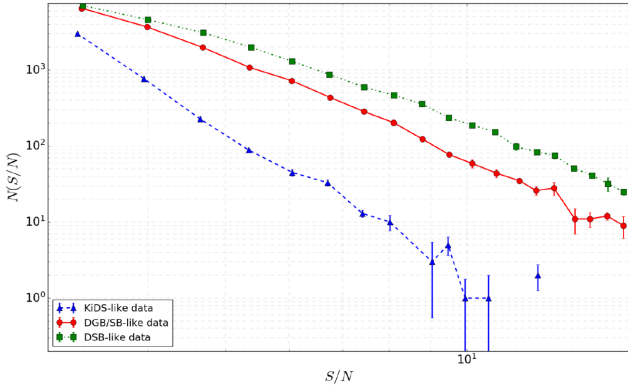
Figure 13. The high S/N peak distributions for n_{\text{eff}} = 9, 30, and 60 \text{gal arcmin}^{-2} (the triangle, circle, and square markers, respectively). The error bars are the variance in the S/N bins for different noise realizations. Note that in some of the high S/N KiDS-like bins there are no detected peaks.
