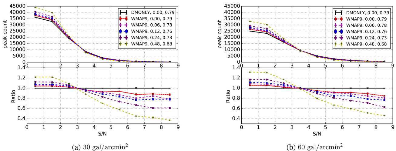
Figure 6. Impact of baryonic physics and neutrino mass, M_\nu = 0.00, 0.06, 0.12, 0.24, and 0.48 eV models, all with fiducial baryonic physics, on the S/N peak distributions from DGB/SB ( 30 \text{ gal arcmin}^{-2} ) and DSB ( 60 \text{ gal arcmin}^{-2} ) surveys based on WMAP 9 cosmology. The legend goes as Cosmology, M_\nu (eV), and S_8 . The comparisons in the bottom panels are with respect to the DMONLY (collisionless dynamics) model with zero neutrino mass. The error bars show the variance of the five different shape noise realizations. In this figure we extend the S/N from 0 to 10 in nine bins in order to assess the impact at high S/N. Note that the amplitudes of the peak counts are different from Figs 3(b) and 4(b) due to wider binning.
