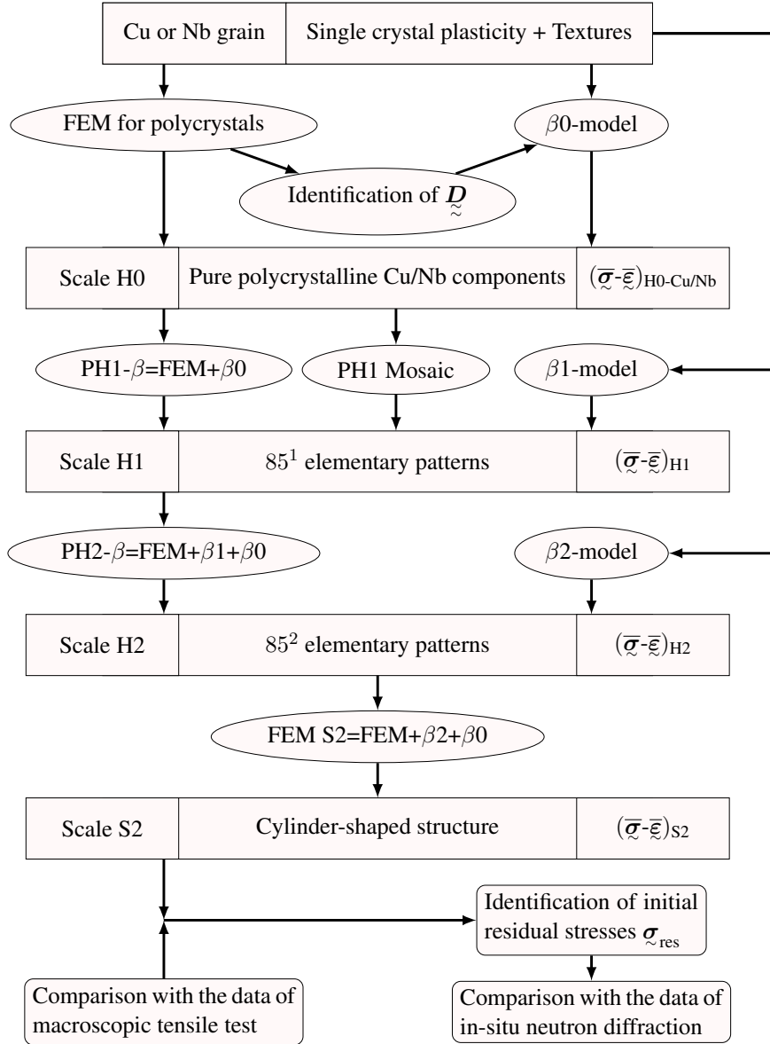
Figure 4: Overview chart of the iterative scale transition steps and experimental comparison. The considered scales and scale transition models are mentioned, together with the obtained effective behavior. The identification of initial residual stresses is also shown. The same parameter combination of D_{ij} is used for all the \beta_i -model ( i=0,1,2 ), once identified at scale H0.
