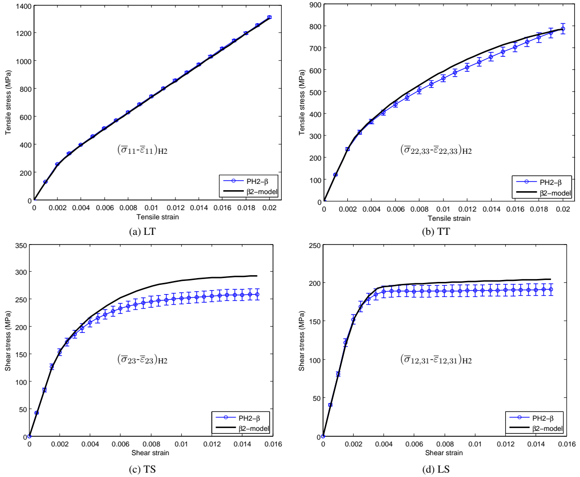
Figure 13: Effective elasto-plastic behavior at scale H2, obtained by the PH2- \beta and \beta 2-model for various loading conditions: (a) LT, (b) TT, (c) TS and (d) LS tests.
