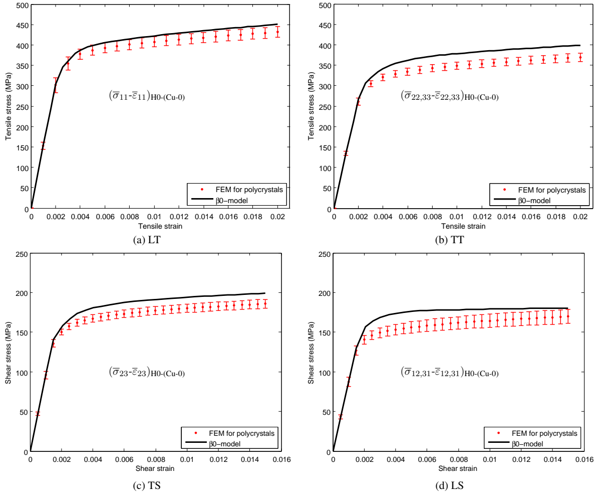
Figure 8: Effective elasto-plastic behavior of the polycrystalline Cu-0, i.e. at scale H0-(Cu-0), obtained by the FEM for polycrystals and the \beta_0 -model. Various loading conditions are presented: (a) Longitudinal Tensile (LT) test, (b) Transverse Tensile (TT) test, (c) Transverse Shear (TS) test and (d) Longitudinal Shear (LS) test. See Section 4.2 for the conventions of loading conditions.
