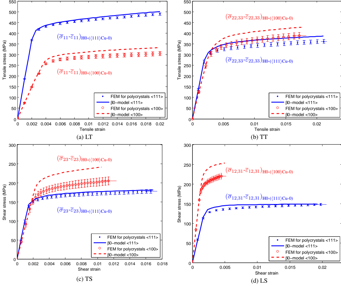
Figure 9: Effective behavior of the individual \langle 111 \rangle and \langle 100 \rangle fiber textures at scale H0-(Cu-0), obtained by the FEM for polycrystals and the \beta_0 -model. Various loading conditions are considered: (a) LT, (b) TT, (c) TS and (d) LS tests. Blue stands for the \langle 111 \rangle fiber texture and red for \langle 100 \rangle .
