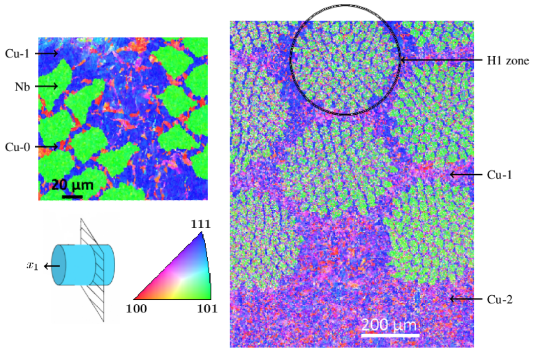
Figure 2: EBSD map in the x_2 - x_3 transverse plane showing Cu and Nb grain orientations (Medy, 2016). Inverse pole figure ( x_1 axis) coloring according to the cubic crystal system. Nb appears in green due to the strong \langle 110 \rangle fiber texture and Cu in red/blue. The specimen diameter is 4.50 mm.
