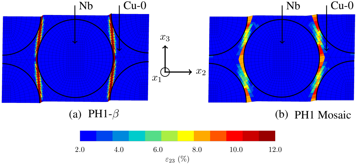
Figure 12: Shear strain \varepsilon_{23} distribution predicted by the (a) PH1- \beta and (b) PH1 Mosaic models at scale H1 with an overall effective transverse shear (\bar{\varepsilon}_{23})_{H1}=1.5\% imposed in the TS test.
