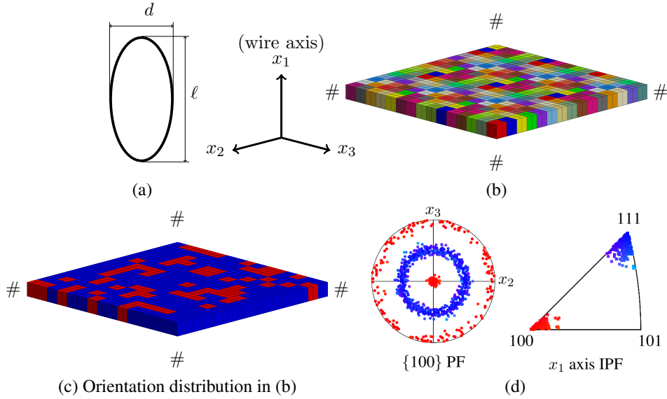
Figure 5: FE meshes for columnar polycrystals: (a) The overall (mean) shape of a single grain elongated along direction x_1 with dimensions \ell \times d \times d ; (b) Parallelepipedic tessellation of 225 grains ( = 15 \times 15 ) with the aspect ratio \ell/d \rightarrow \infty (periodic boundary conditions, denoted #, are considered); (c) Orientation distribution in the tessellation mesh (b), blue stands for \langle 111 \rangle fiber texture and red for \langle 100 \rangle ; (d) \{100\} Pole Figure and x_1 axis Inverse Pole Figure of Cu-0. Grain orientations are generated by the software LaboTex based on experimental EBSD textures.
