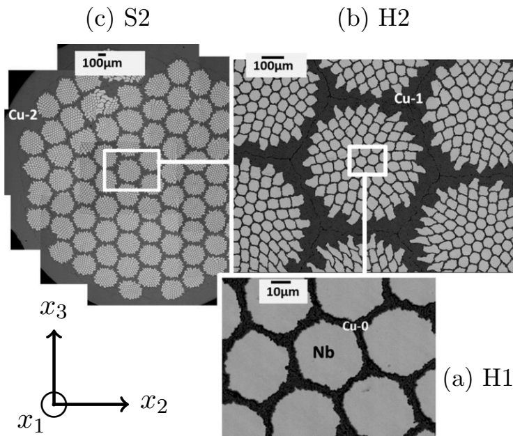
Figure 1: Successive section views of the Cu-Nb nano-composite wires containing 85^2 elementary Cu/Nb long fibers. The diameter of specimen (c) is reduced from actual 4.50 mm to two smaller diameters by supplementary cold-drawing: 2.10 mm for in-situ neutron diffraction experiments and 0.29 mm for macroscopic tensile tests in this work. The smaller scale for pure polycrystalline Cu or Nb (i.e. scale H0) is not shown in this figure. See Section 2.3 for scale conventions and notations.
