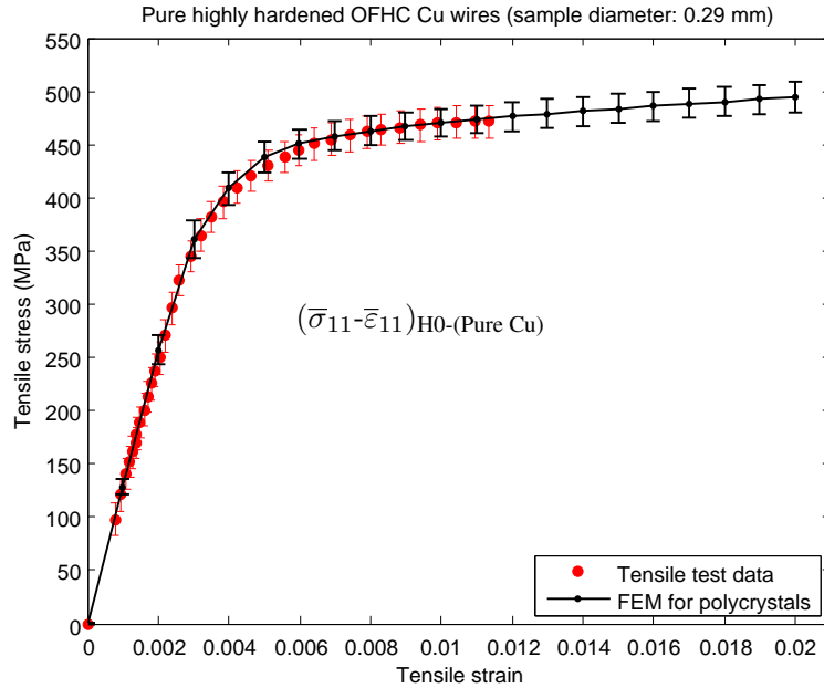
Figure 7: Identification of phenomenological parameters for single crystal plasticity: FEM results are compared to experimental data for the pure highly hardened OFHC Cu aggregate.
