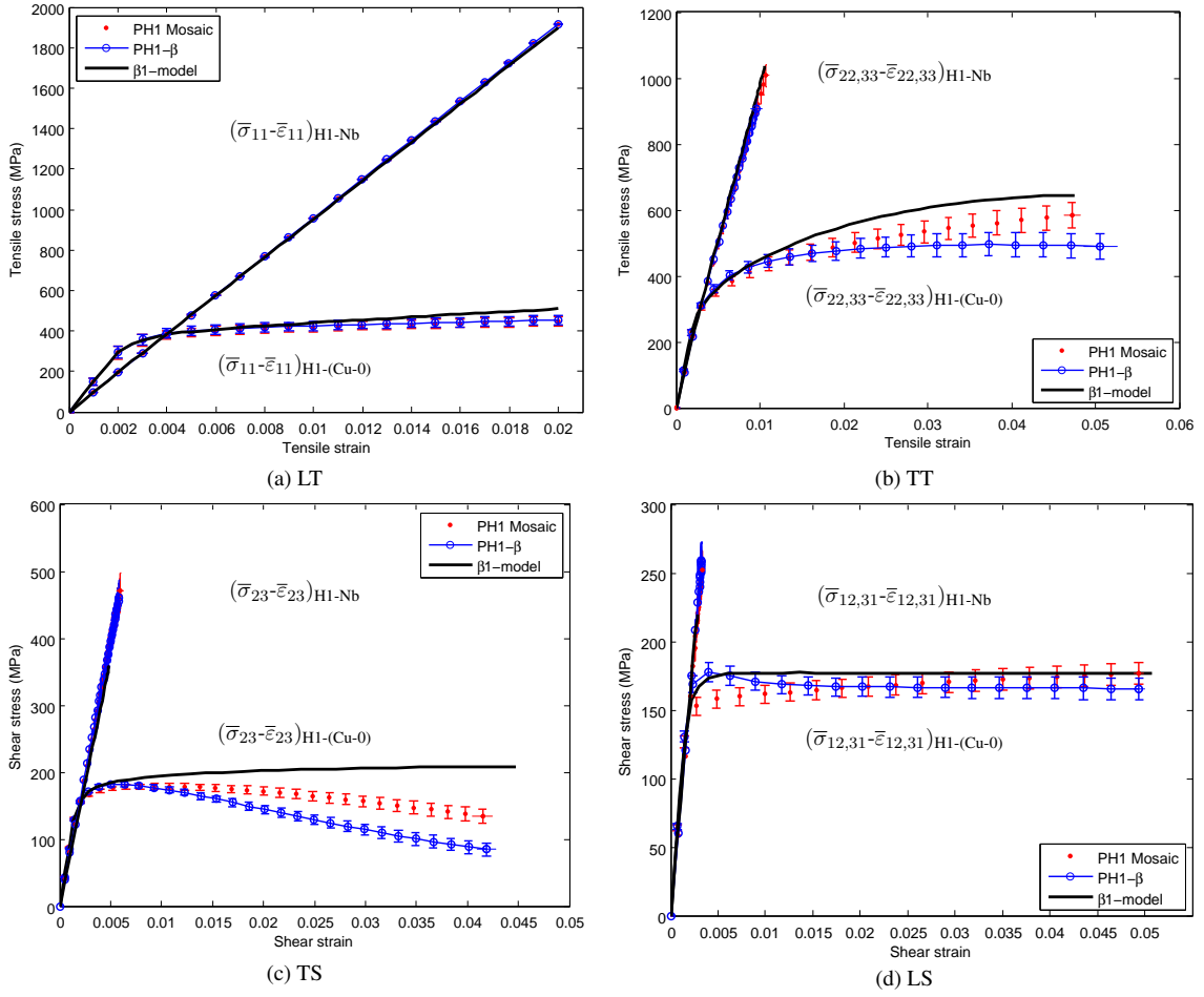
Figure 11: Effective behavior of the individual Cu-0 and Nb components at scale H1, obtained by the PH1 Mosaic, PH1- \beta , and \beta 1-model approaches. Various loading conditions are presented: (a) LT, (b) TT, (c) TS and (d) LS tests.
