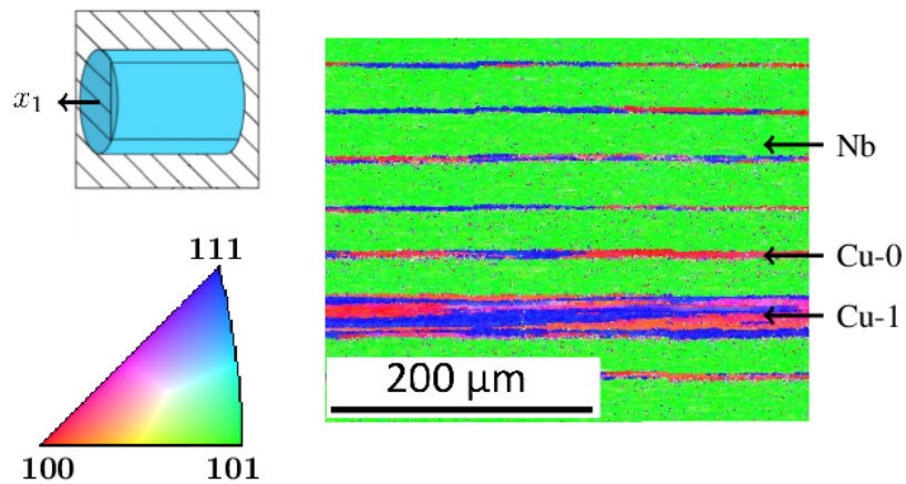
Figure 3: EBSD map in a plane parallel to x_1 showing Cu and Nb grain orientations (Medy, 2016). Inverse pole figure ( x_1 axis) coloring according to the cubic crystal system. The specimen diameter is 4.50 mm. Highly elongated grains along x_1 are observed for all components (e.g. Cu-1 in this figure).
