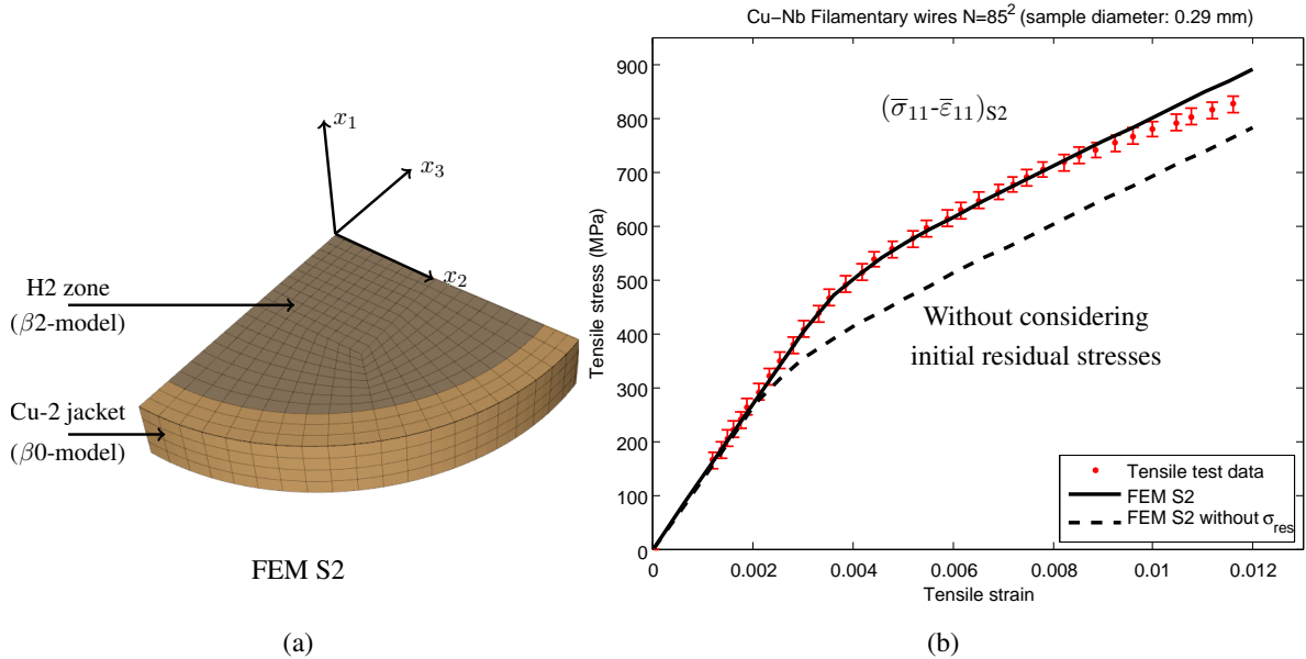
Figure 15: (a) 1/4th FEM mesh of a cross-section of the S2 sample (the 3 elements in thickness are for illustration purposes since results are invariant along the wire length, i.e. cross-section thickness); (b) Experimental comparison for the monotonic LT test at S2. The dashed line in (b) shows the model prediction without taking into account the initial residual stresses.
