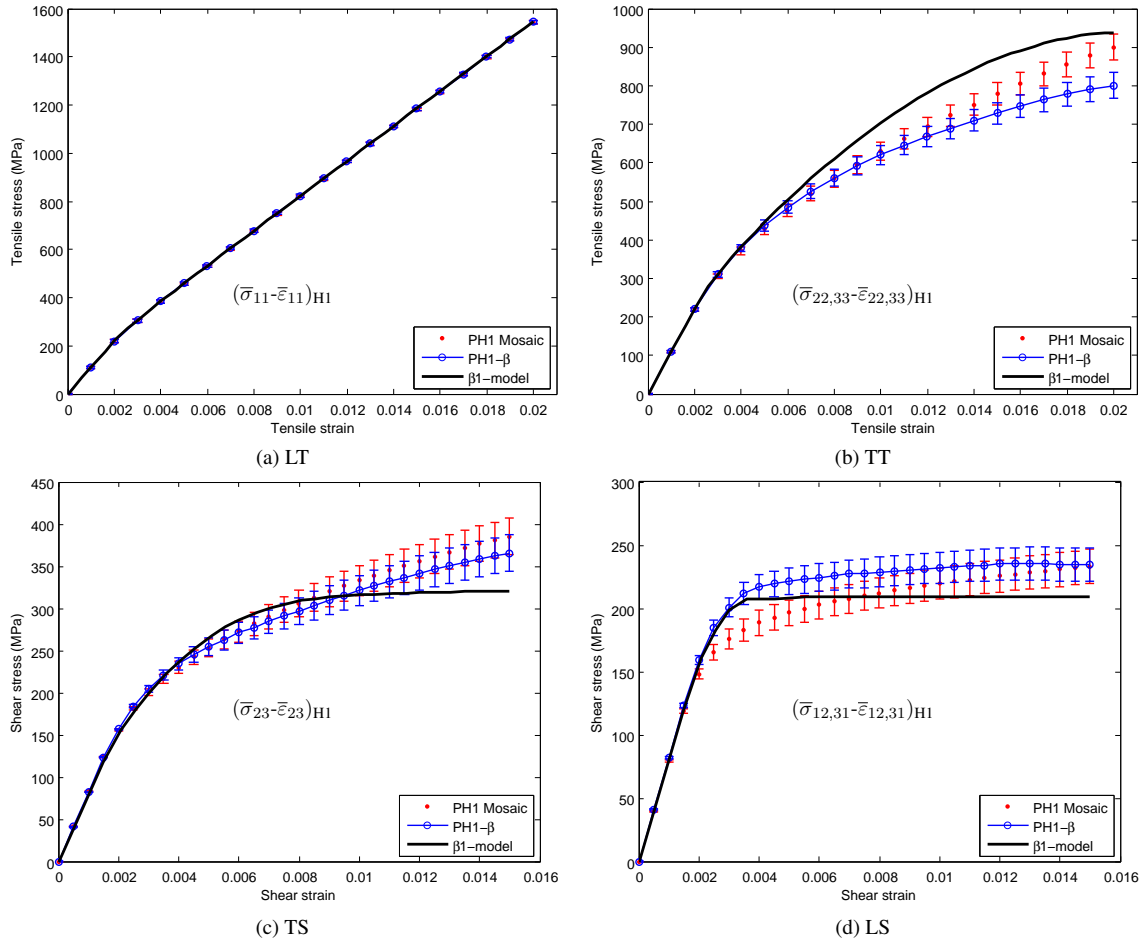
Figure 10: Effective elasto-plastic behavior at scale H1, obtained by the PH1 Mosaic, PH1- \beta , and \beta 1-model. Various loading conditions are presented: (a) LT, (b) TT, (c) TS and (d) LS tests.
