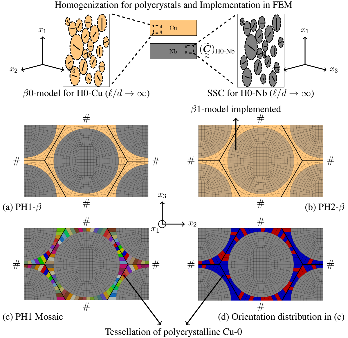
Figure 6: Multiscale modeling of effective elasto-plastic behavior of Cu-Nb wires (Orange stands for Cu, gray for Nb, light gray for Cu-Nb composite): (a) Using the PH1- \beta at scale H1, a periodic distribution of Nb fibers is assumed (# denotes periodic boundary conditions). The polycrystalline Nb and Cu-0 aggregates are described by an effective elastic stiffness obtained by the SSC scheme and an elasto-plastic behavior provided by the \beta_0 -model, respectively (see the inset). (b) Using the PH2- \beta at scale H2, the behavior of the Cu-Nb composite H1 zone is provided by the \beta_1 -model, while that of the polycrystalline Cu-1 aggregate is given by a \beta_0 -model accounting for the microstructure of Cu-1. (c) Using the PH1 Mosaic at scale H1, polycrystalline Cu-0 surrounding the elastic Nb is described by a tessellation of polycrystalline aggregates. (d) Orientation distribution in the tessellation of (c), blue stands for the \langle 111 \rangle fiber texture and red for \langle 100 \rangle .
