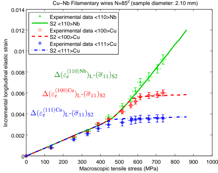
Figure 16: Experimental comparison with the in-situ neutron diffraction tensile experiments (data obtained by Medy (2016)): applied macroscopic monotonic longitudinal stress (\bar{\sigma}_{11})_{S2} vs. incremental longitudinal mean elastic strains of individual \langle 111 \rangle Cu, \langle 100 \rangle Cu and \langle 110 \rangle Nb fiber textures, i.e. \Delta(\varepsilon_e^{\langle 111 \rangle \text{Cu}})_L , \Delta(\varepsilon_e^{\langle 100 \rangle \text{Cu}})_L and \Delta(\varepsilon_e^{\langle 110 \rangle \text{Nb}})_L .
