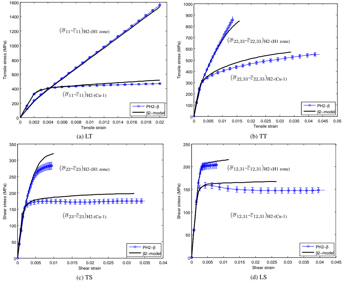
Figure 14: Effective behavior of the individual H1 zones and Cu-1 components at scale H2, obtained by the PH2- \beta and \beta 2-model for various loading conditions: (a) LT, (b) TT, (c) TS and (d) LS tests.
