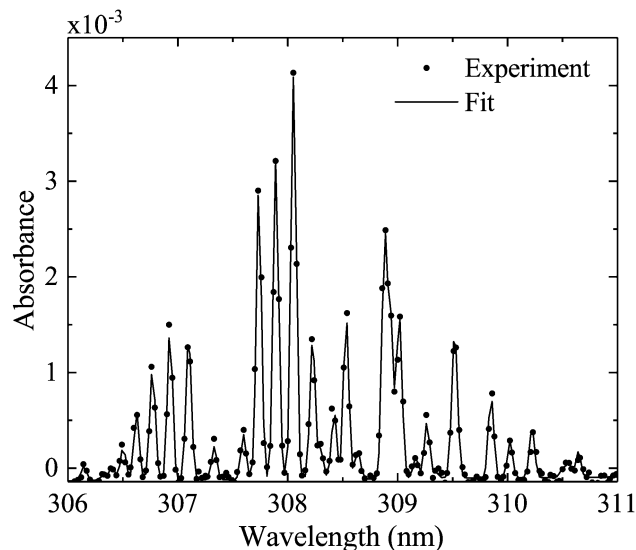
Fig. 6 Example spectrum for the measured and fitted transition \text{OH}(X^2\Pi_j, v' = 0) \rightarrow \text{OH}(A^2\Sigma^+, v'' = 0) using the UV-BBAS I setup, for 4 slm dry and 1 slm humidified He, 530 V pp . The calculated \text{OH}(X^2\Pi_j, v' = 0) density obtained from this spectrum is 2.6 \times 10^{14} \text{ cm}^{-3} .
