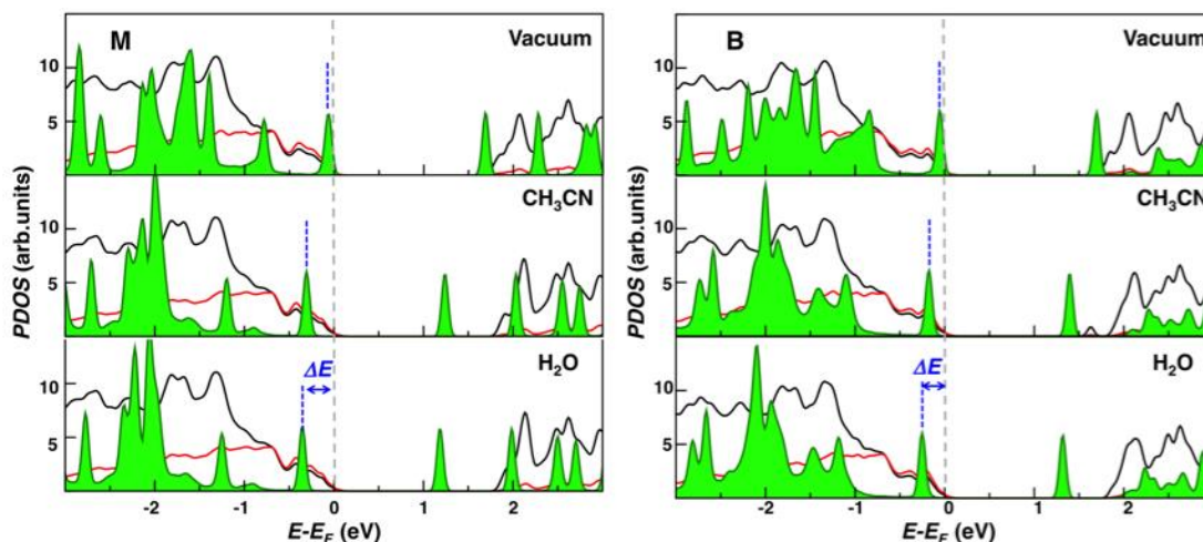
Figure 3. Projected density of states (PDOS) at the DFT-PBE+U level of theory for Ni d states (black line), ONiO p states (red line) and T1 dye (green line) in the M and B adsorption mode calculated in vacuum (top panels), acetonitrile (central panels) and water (bottom panels). The Fermi energy ( E_F ) is set to zero. Corresponding \Delta E values are reported in Table 1.
