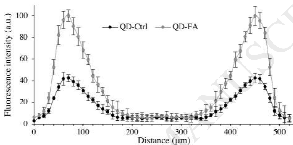
Figure 5. Mean fluorescence distribution profiles of QD-Ctrl and QD-FA across the KB spheroid cut after 4h incubation with QDs.
