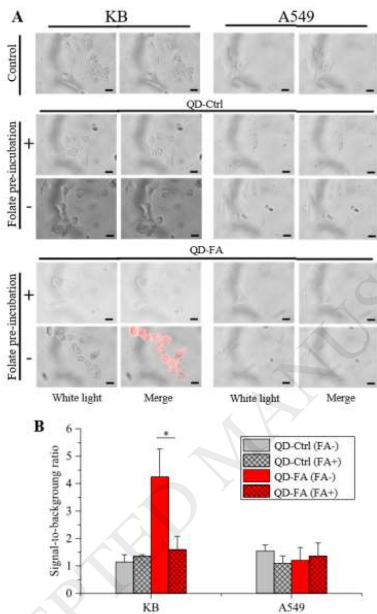
Figure 4. (A) The images of KB spheroid incubated with QDs for 4 h, with or without folic acid pre-incubation. (B) SBR measured for each condition. The fluorescence was excited at \lambda = 405-445 nm and registered above 590 nm. The QD concentration was 100 nM. Scale bar = 100 \mu m; *: p-value < 0,05
