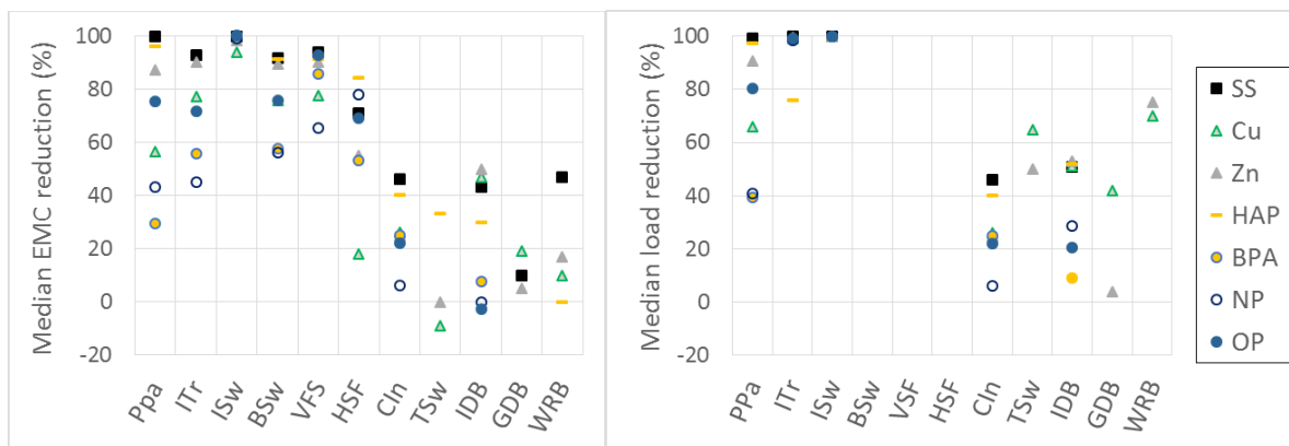
Figure 2 : median EMC and event load reductions per SCM for total fraction
