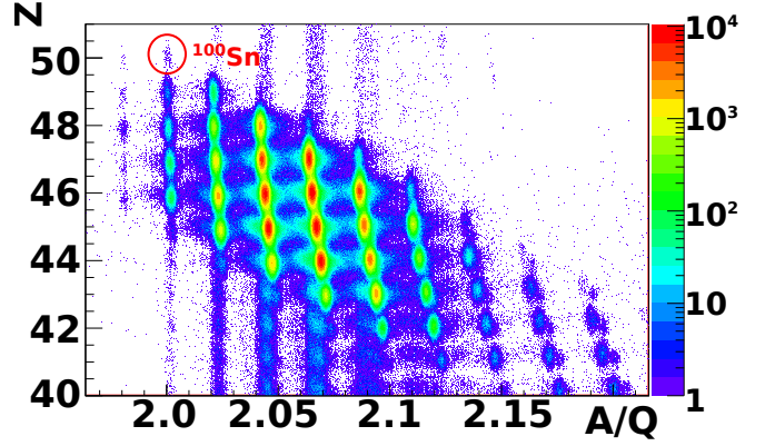
Figure 1. (Colour online) Particle identification plot of secondary ions produced in this experiment and implanted in the active stopper detector at the end of the ZeroDegree spectrometer (see text for details). Events from the identification of ^{100}\text{Sn} isotopes are highlighted as a reference.
