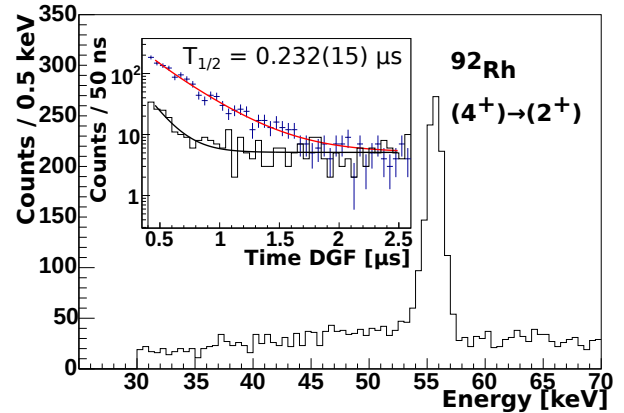
Figure 4. (Colour online) Time-delayed projected \gamma -ray energy between 400\text{ ns} \leq T_{DGF} \leq 1200\text{ ns} . The inset shows the time spectrum and decay curve of the 55 keV transition. Note that this time spectrum was generated by increasing the upper time limit to T_{DGF} \leq 3500\text{ ns} .
