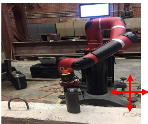
Figure 4. Robotic Impact Echo (IE)
